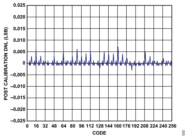
Figure 34. AD9714 Postcalibration DNL at 1.8 V
