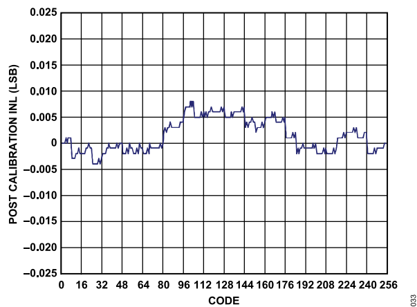
Figure 35. AD9714 Postcalibration INL at 3.3 V
