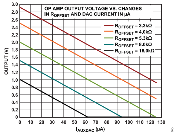
Figure 108. AUXDAC Op Amp Output vs. Current, AVDD = 3.3 V, No Load, AUXDAC 0x1FF to 0x000
