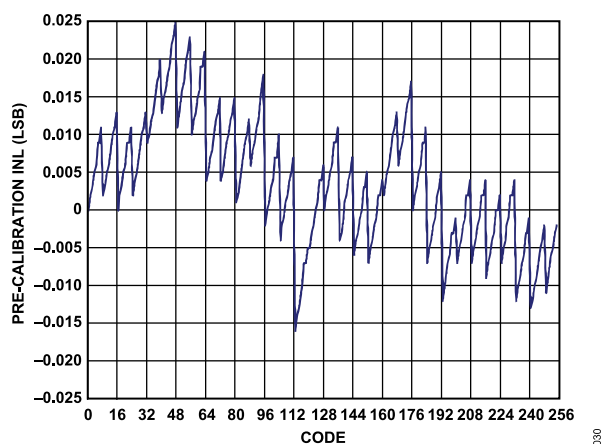
Figure 32. AD9714 Precalibration INL at 3.3 V
