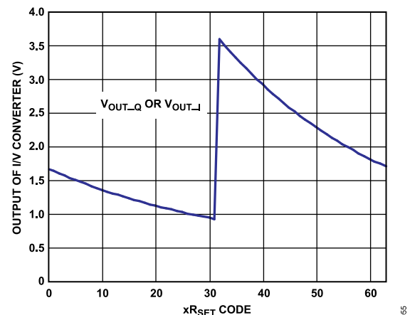
Figure 100. Effect of xR_{SET} Code
