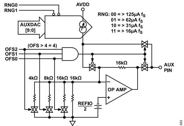
Figure 107. AUXDAC Simplified Circuit Diagram
