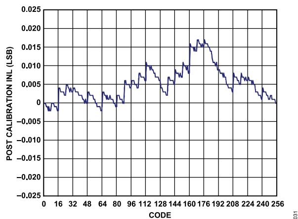
Figure 33. AD9714 Postcalibration INL at 1.8 V
