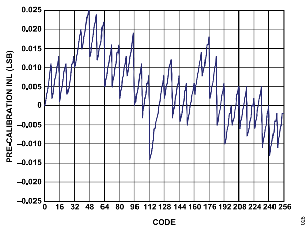
Figure 30. AD9714 Precalibration INL at 1.8 V
