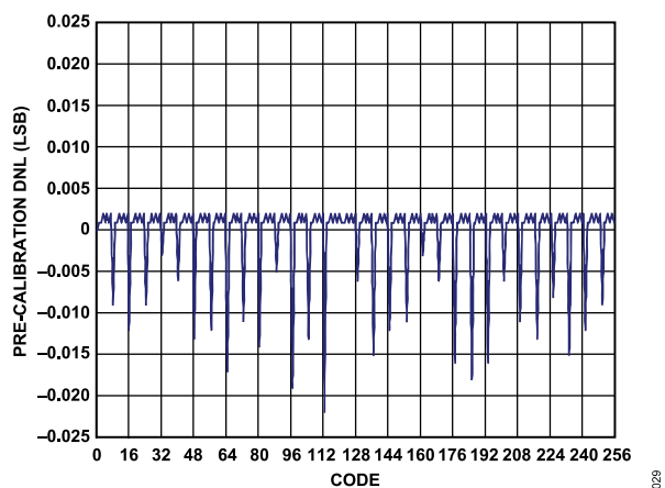
Figure 31. AD9714 Precalibration DNL at 1.8 V
