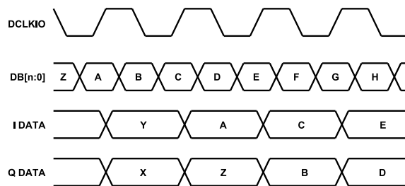
Figure 89. Timing Diagram with IFIRST = 0, IRISING = 0
