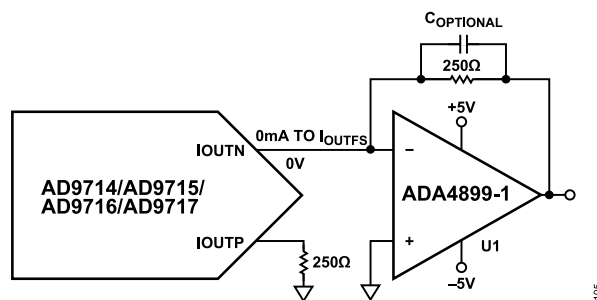
Figure 105. Unipolar Buffered Voltage Output
