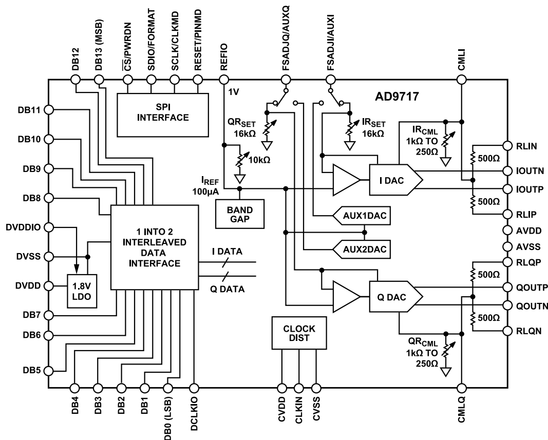
Figure 84. Simplified Block Diagram
