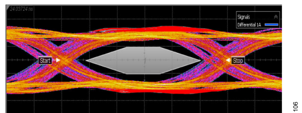
Figure 106. Digital Outputs Data Eye, External 100 \Omega Terminations at 16 Gbps
