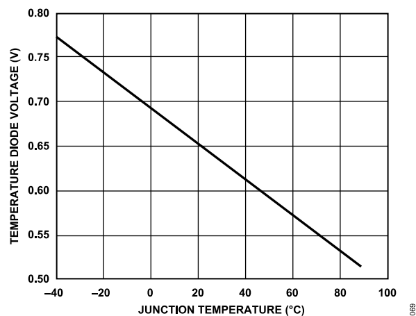
Figure 73. Typical Voltage Response of the 1× Temperature Diode
