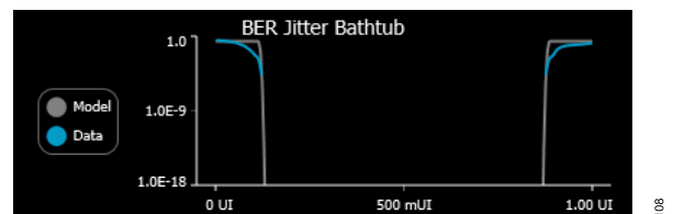
Figure 108. Digital Outputs Bathtub Curve, External 100 \Omega Terminations at 16 Gbps
