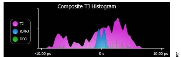
Figure 107. Digital Outputs Jitter Histogram, External 100 \Omega Terminations at 16 Gbps
