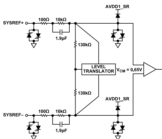
Figure 43. SYSREF± Inputs
