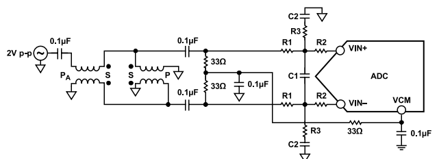
Figure 50. Differential Double Balun Input Configuration
