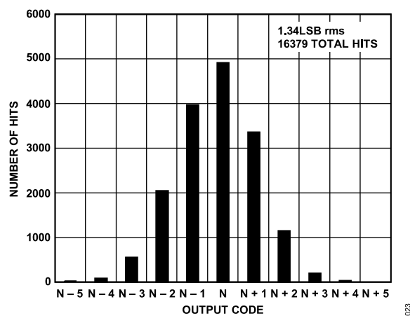
Figure 16. AD9643-170 Grounded Input Histogram
