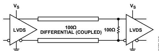
Figure 74. LVDS Output Termination
