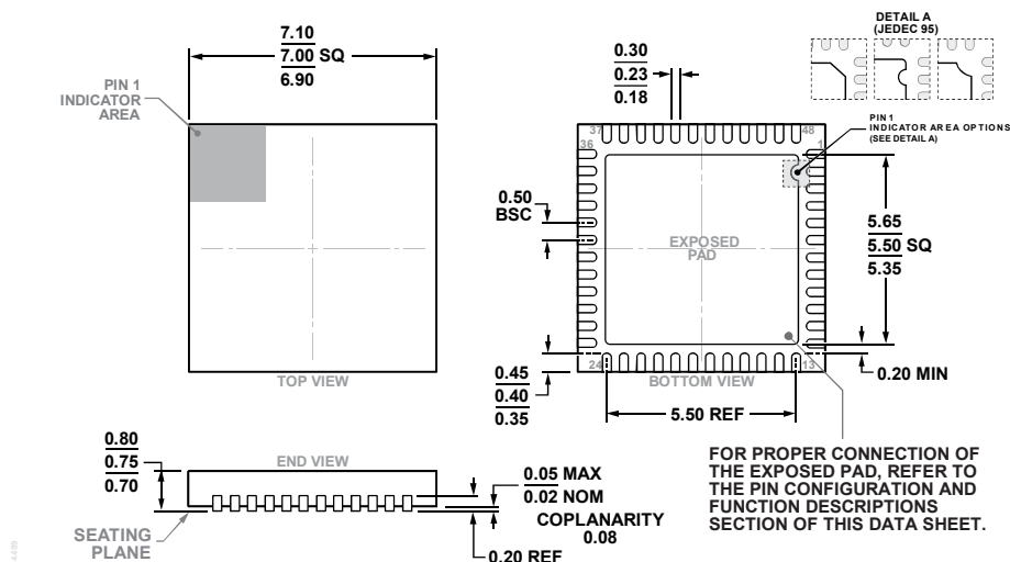
Figure 85. 48-Lead Lead Frame Chip Scale Package [LFCSP] 7 mm x 7 mm Body and 0.75 mm Package Height (CP-48-9)
