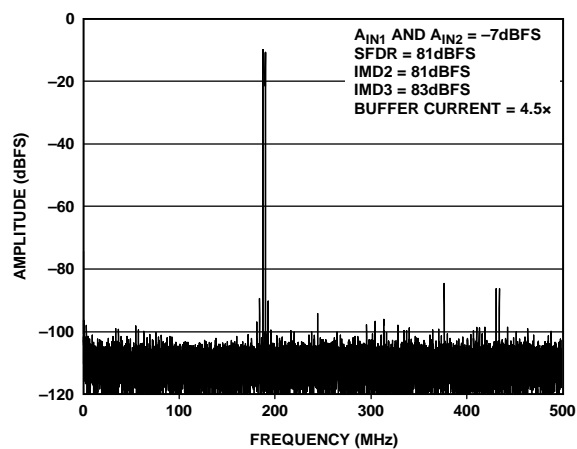
Figure 18. Two-Tone FFT; f_{IN1} = 184\text{ MHz} , f_{IN2} = 187\text{ MHz}
