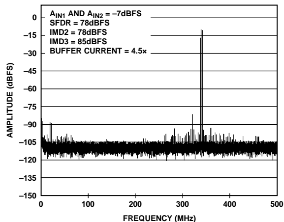
Figure 19. Two-Tone FFT; f_{IN1} = 338\text{ MHz} , f_{IN2} = 341\text{ MHz}
