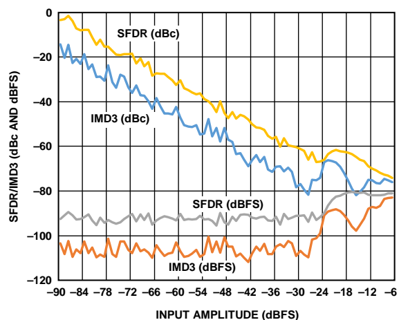
Figure 20. Two-Tone SFDR/IMD3 vs. Input Amplitude ( A_{IN} ) with f_{IN1} = 184\text{ MHz} and f_{IN2} = 187\text{ MHz}
