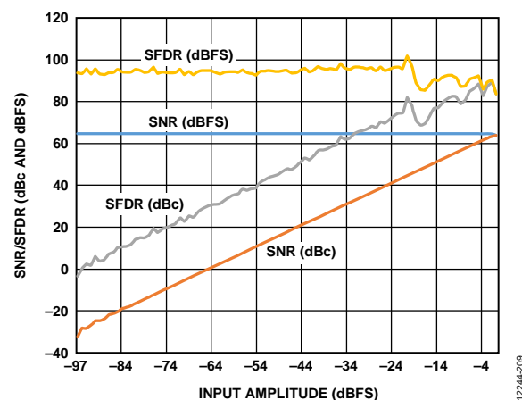
Figure 22. SNR/SFDR vs. Analog Input Level, f_{IN} = 10.3\text{ MHz} ; Buffer Current = 2.0x
