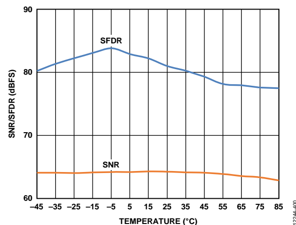
Figure 23. SNR/SFDR vs. Temperature, f_{IN} = 170.3\text{ MHz}
