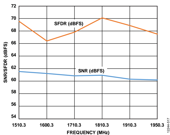
Figure 40. SNR/SFDR vs. Input Frequency; 1500 MHz < f_{IN} < 2000 MHz; Buffer Current = 8.5\times (Uses Circuit Shown in Figure 64)
