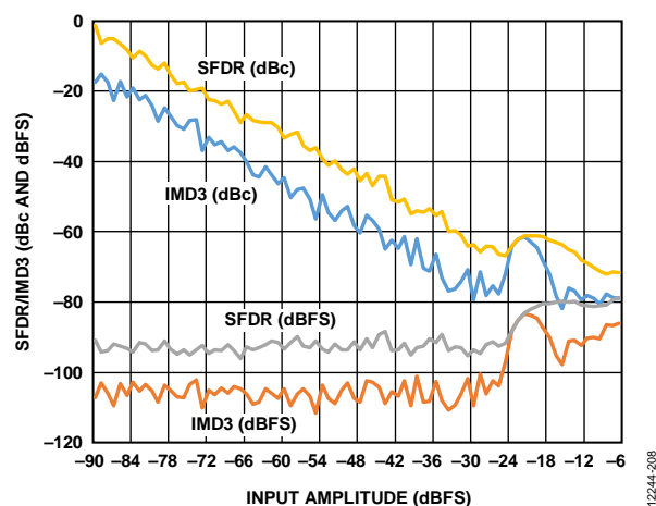
Figure 21. Two-Tone SFDR/IMD3 vs. Input Amplitude ( A_{IN} ) with f_{IN1} = 338\text{ MHz} and f_{IN2} = 341\text{ MHz}
