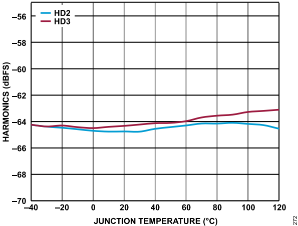
Figure 41. Harmonics vs. Junction Temperature, f_{IN}=1.8\text{ GHz} , A_{IN}=-1\text{ dBFS}
