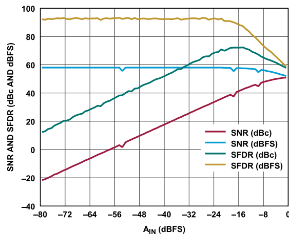
Figure 15. Single-Tone SNR and SFDR vs. A_{IN} at f_{IN} = 3.6 GHz
