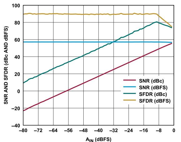
Figure 8. Single-Tone SNR and SFDR vs. A_{IN} at f_{IN} = 450 MHz
