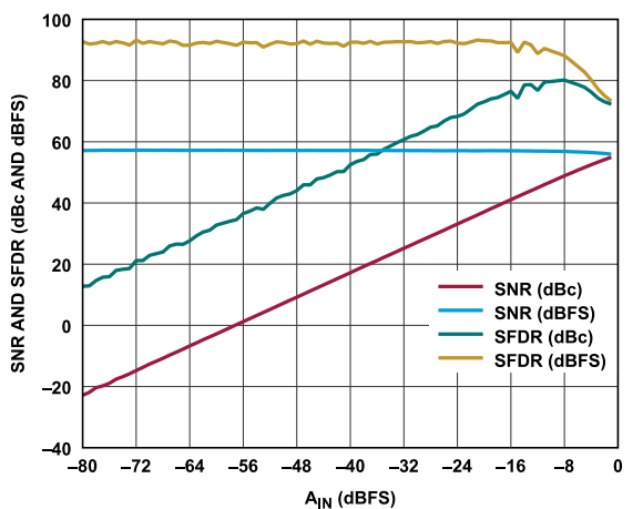
Figure 9. Single-Tone SNR and SFDR vs. A_{IN} at f_{IN} = 900 MHz
