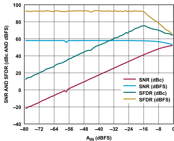
Figure 14. Single-Tone SNR and SFDR vs. A_{IN} at f_{IN} = 2.7 GHz
