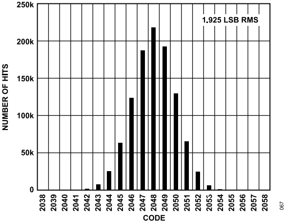
Figure 43. Input Referred Noise Histogram
