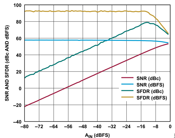
Figure 10. Single-Tone SNR and SFDR vs. A_{IN} at f_{IN} = 1.8 GHz
