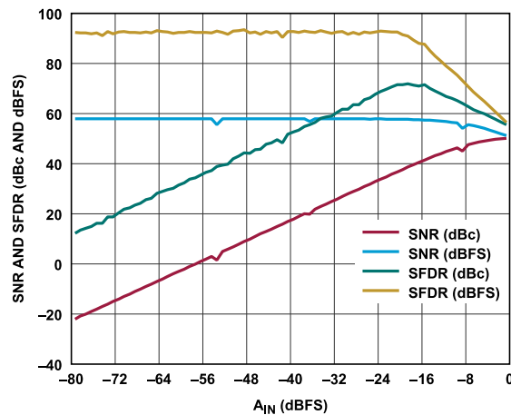
Figure 16. Single-Tone SNR and SFDR vs. A_{IN} at f_{IN} = 4.5 GHz
