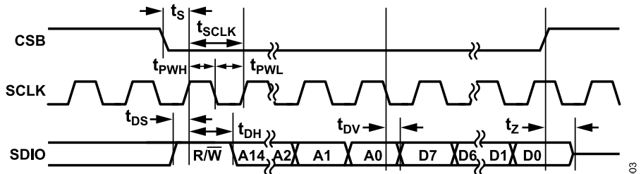
Figure 2. Timing Diagram for 3-Wire Read Operation
