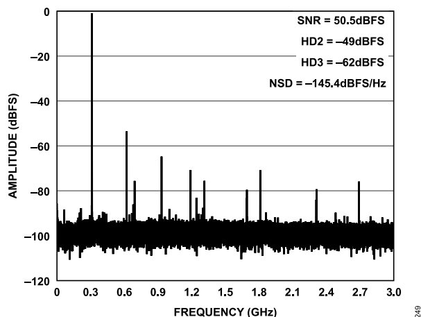
Figure 18. Single-Tone FFT at f_{IN} = 6.3 GHz
