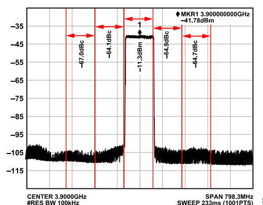
Figure 35. ACLR Performance for 100 MHz 5G Test Vector at f_{OUT} = 3.9 GHz and f_{DAC} = 11.898 GSPS, Test Vector Peak to RMS = 11.7 dB with -1 dBFS Backoff (Mode 9C), Channel Interpolation 3 \times , Main Interpolation 8 \times
