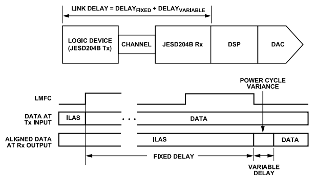
Figure 55. JESD204B Link Delay = Fixed Delay + Variable Delay
