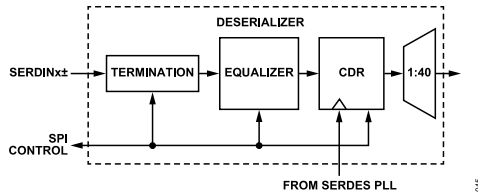
Figure 45. Deserializer Block Diagram
