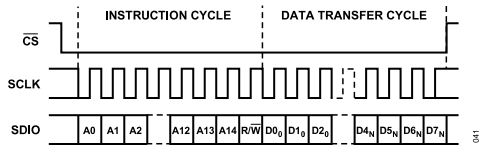
Figure 41. Serial Register Interface Timing, LSB First, Register 0x000, Bit 6 and Bit 1 = 1
