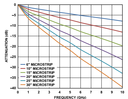
Figure 50. Insertion Loss of 50 Ω Microstrips on FR4
