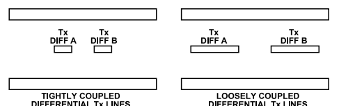
Figure 80. Tightly Coupled vs. Loosely Coupled Differential Traces
