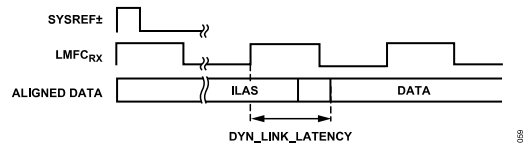
Figure 59. DYN_LINK_LATENCY_x Illustration
