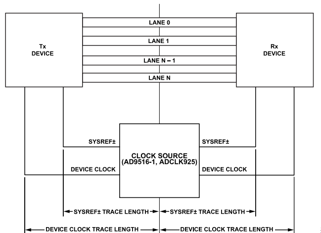
Figure 81. \text{SYSREF}_{\pm} Signal and Device Clock Trace Length
