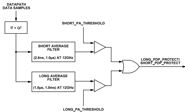
Figure 70. PDP Block Diagram
