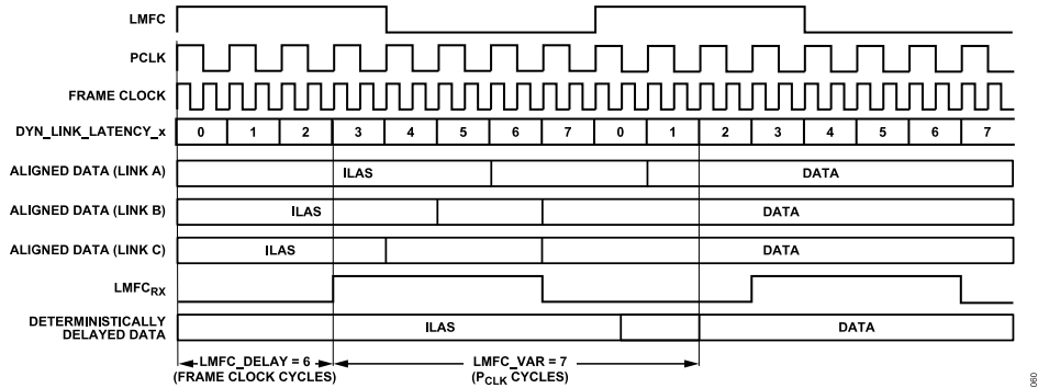
Figure 60. Multilink Synchronization Settings, Derived Method Example
