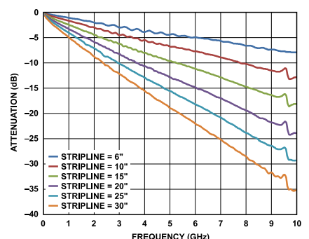
Figure 49. Insertion Loss of 50 Ω Striplines on FR4
