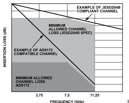
Figure 48. Insertion Loss Allowed
