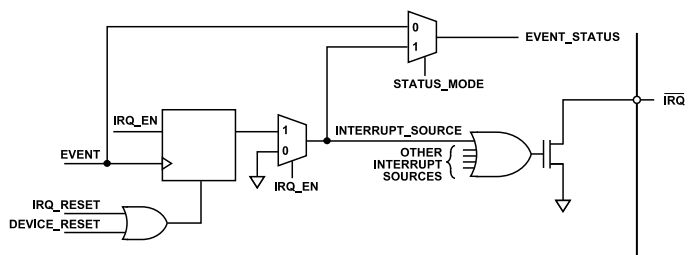
Figure 77. Simplified Schematic of \overline{\text{IRQx}} Circuitry
