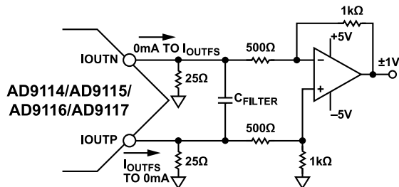
Figure 105. Differential Buffered Voltage Output
