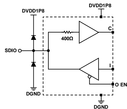
Figure 50. SDIO Input/Output
