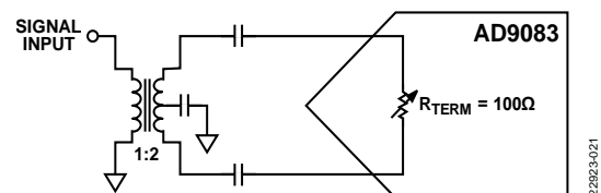
Figure 58. AC-Coupled Inputs to the AD9083 Using a Transformer
