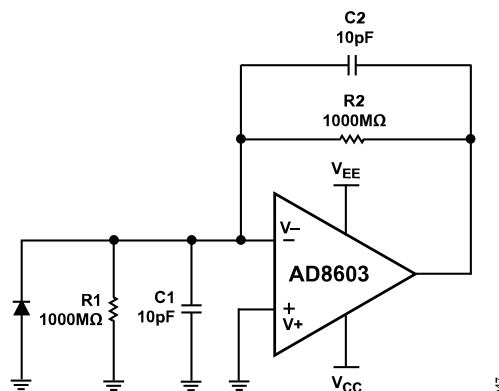
Figure 47. Photodiode Circuit
