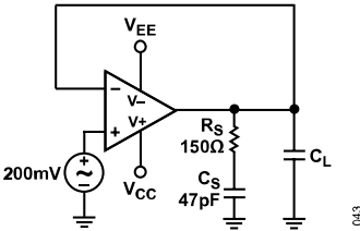
Figure 43. Snubber Network
