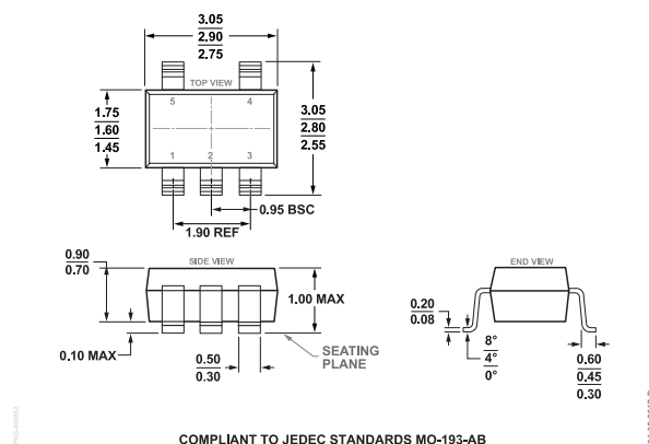
Figure 48. 5-Lead Thin Small Outline Transistor Package [TSOT] (UJ-5) Dimensions shown in millimeters
