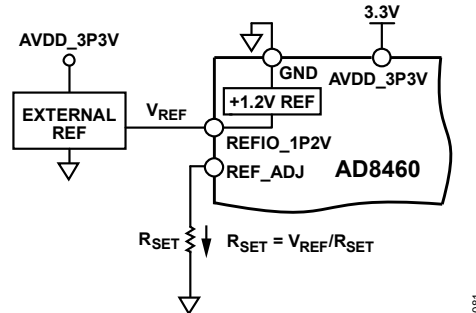
Figure 61. External Reference Configuration
