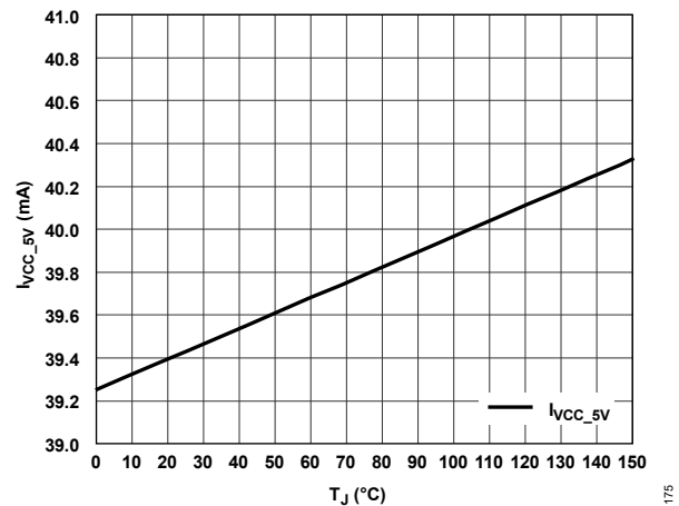
Figure 55. VCC_5V Quiescent Supply Current vs. Temperature, V_{CC\_5V} = 5 V
