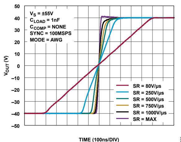
Figure 2. Large Signal Pulse Response vs. Edge Speed with External Slew Control
