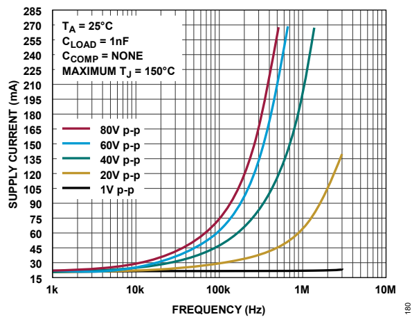
Figure 52. Supply Current and Amplitude vs. Frequency Square Wave, with Heatsink and Airflow, C_{LOAD} = 1 nF, C_{COMP} = \text{None}
