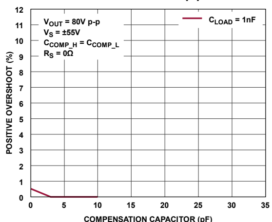
Figure 24. Large Signal Pulse Response Overshoot vs. C_{LOAD} and C_{COMP} , Positive Overshoot
