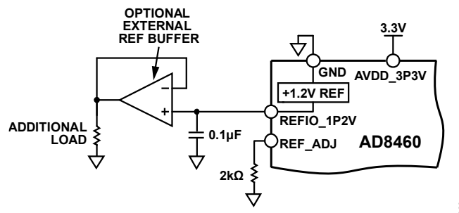
Figure 60. Buffered Internal Reference Configuration
