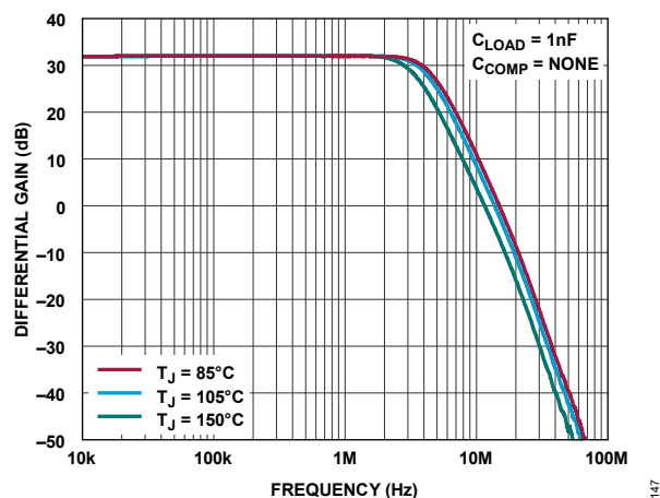
Figure 32. Small Signal Frequency Response vs. Temperature, C_{LOAD} = 1 nF, C_{COMP} = None
