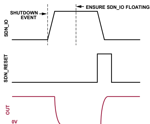
Figure 66. Shutdown Response Sequence
