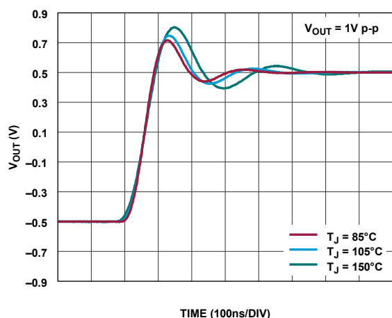
Figure 22. Pulse Response vs. Temperature, Rising Edge, V_{OUT} = 1\text{ V p-p}
