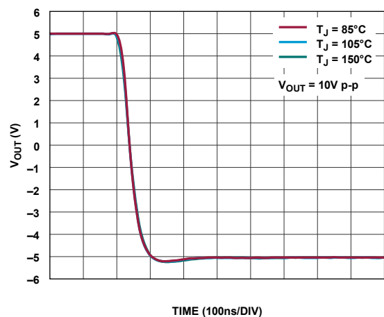
Figure 19. Pulse Response vs. Temperature, Falling Edge, V_{OUT} = 10\text{ V p-p}
