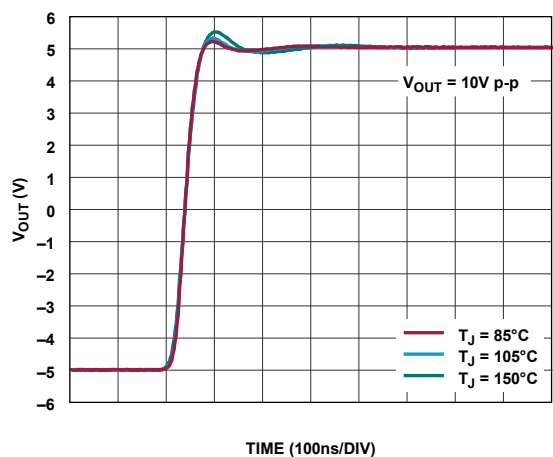
Figure 20. Pulse Response vs. Temperature, Rising Edge, V_{OUT} = 10\text{ V p-p}
