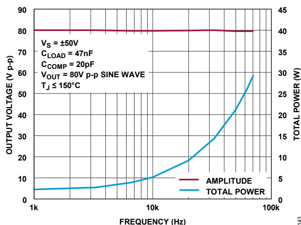
Figure 28. Large Signal Bandwidth, C_{LOAD} = 47 nF, C_{COMP} = 20 pF
