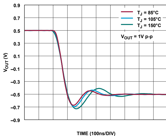
Figure 21. Pulse Response vs. Temperature, Falling Edge, V_{OUT} = 1\text{ V p-p}
