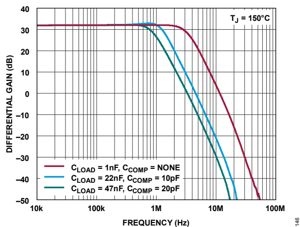
Figure 29. Small Signal Frequency Response vs. C_{LOAD} , T_J = 150^\circ C
