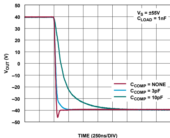
Figure 9. Falling Edge - Large Signal Pulse Response vs. C_{COMP} , Falling Edge, C_{LOAD} = 1 nF
