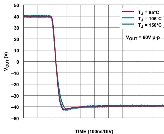
Figure 17. Pulse Response vs. Temperature, Falling Edge, V_{OUT} = 80\text{ V p-p}
