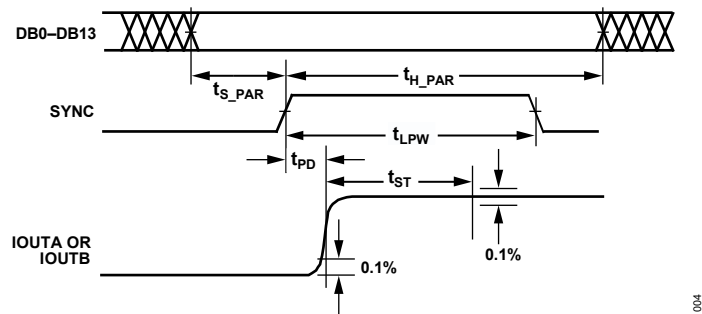
Figure 4. Parallel Inputs Timing Diagram
