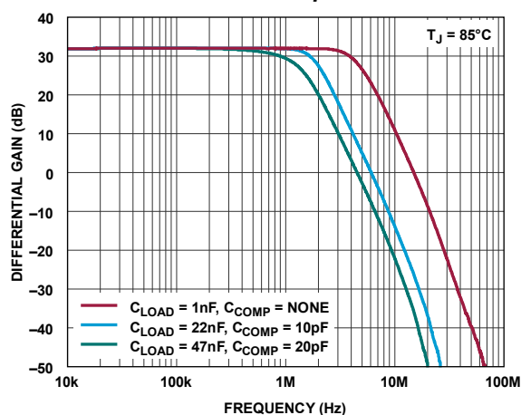
Figure 27. Small Signal Frequency Response vs. C_{LOAD} , T_J = 85^\circ\text{C}
