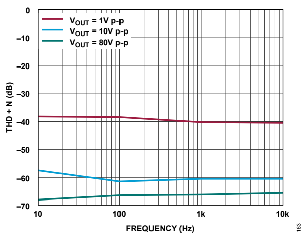
Figure 41. Total Harmonic Distortion and Noise vs. Frequency at Various Large Output Swings
