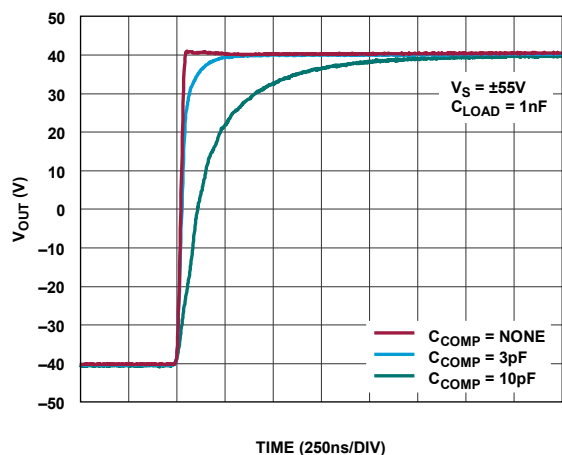
Figure 8. Large Signal Pulse Response vs. C_{COMP} , Rising Edge, C_{LOAD} = 1 nF
