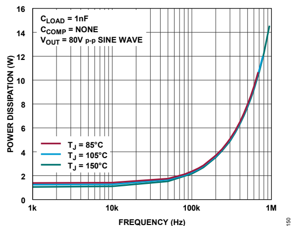
Figure 33. Large Signal Frequency Response vs. Temperature, C_{LOAD} = 1 nF, C_{COMP} = None
