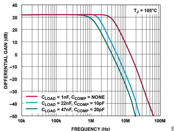
Figure 30. Small Signal Frequency Response vs. C_{LOAD} , T_J = 105^\circ C
