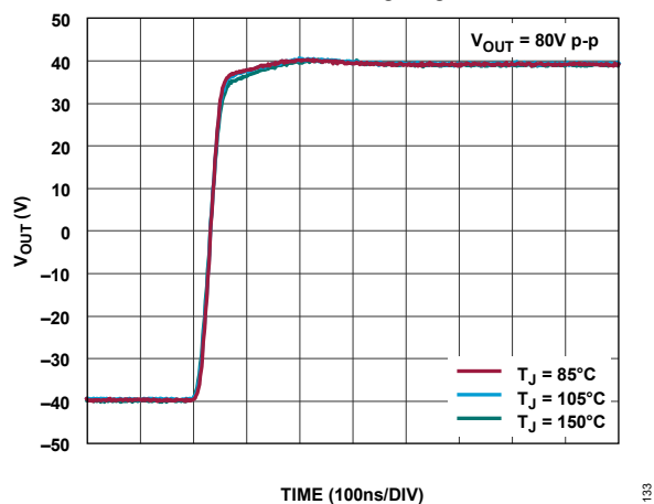
Figure 18. Pulse Response vs. Temperature, Rising Edge, V_{OUT} = 80\text{ V p-p}
