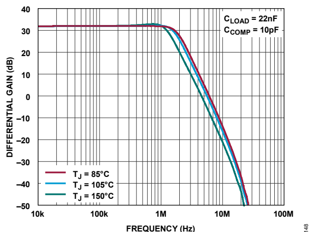
Figure 31. Small Signal Frequency Response vs. Temperature, C_{LOAD} = 22 nF, C_{COMP} = 10 pF
