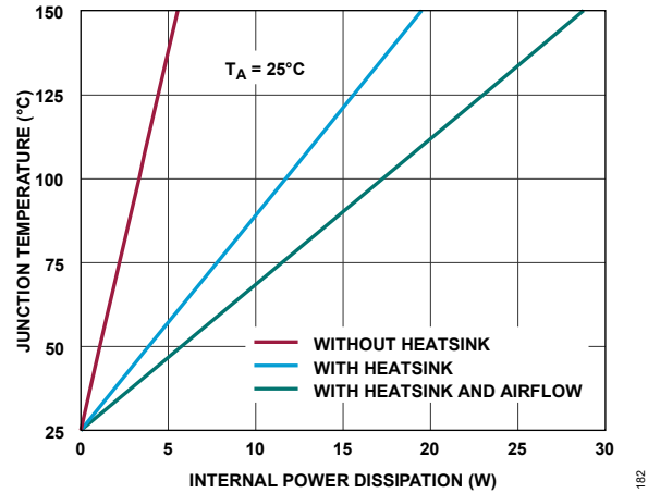
Figure 53. Junction Temperature vs. Internal Power Dissipation
