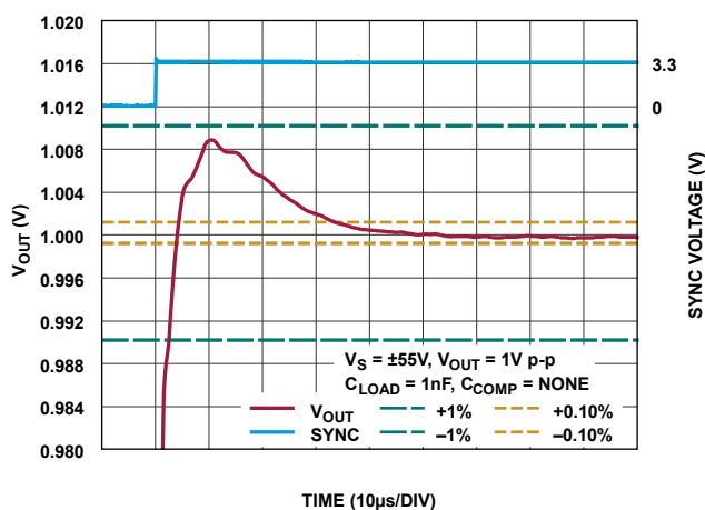
Figure 40. Settling Time to 0.1% and 1%, V_{OUT} = 1 Vp-p, V_S = \pm 55 V, C_{LOAD} = 1 nF, C_{COMP} = \text{None}
