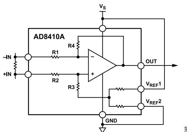
Figure 53. Split Supply
