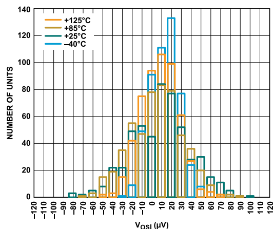
Figure 44. Offset Voltage ( V_{OS} ) Distribution, RTI
