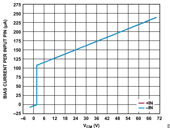
Figure 14. Bias Current Per Input Pin vs. V_{CM} , V_S = 5 V
