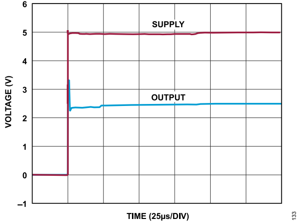
Figure 34. Start-Up Response
