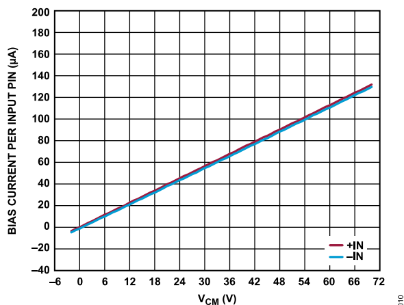
Figure 15. Bias Current Per Input Pin vs. V_{CM} , V_S = 0 V, R_L = 10 kΩ
