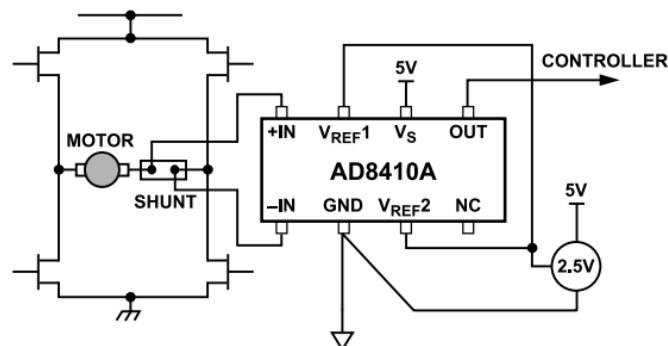
Figure 60.H-Bridge Motor Control
