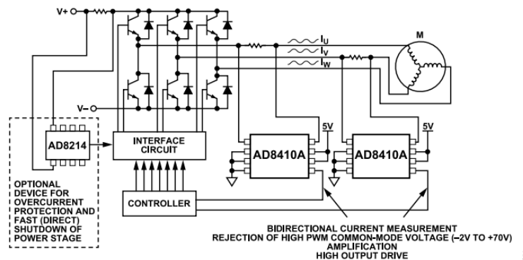
Figure 59.3-Phase Motor Control
