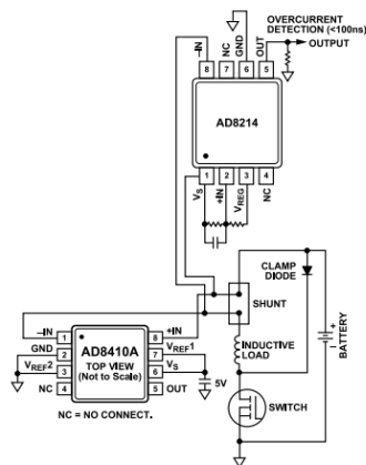
Figure 63. High Rail Current Sensing
