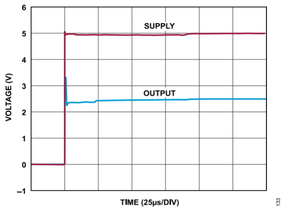
Figure 35. Start-Up Response
