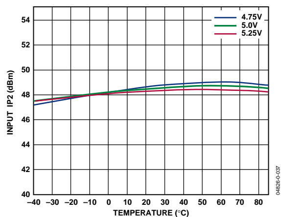
Figure 15. Input IP2 vs. Temperature, F_{RF} = 890 \text{ MHz} , F_{LO} = 1090 \text{ MHz} (RF Tone Spacing = 50 MHz)
