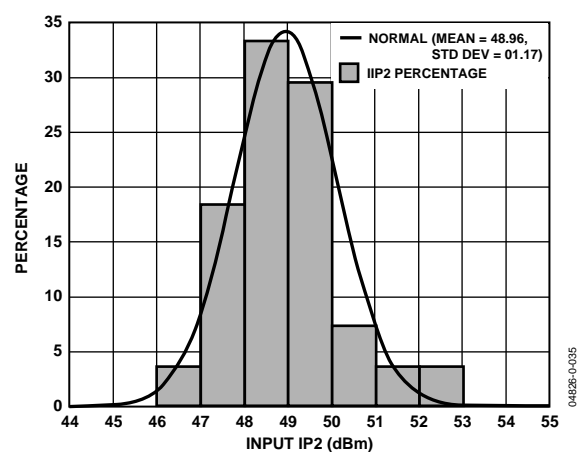
Figure 17. Input IP2 Distribution, F_{RF} = 890 \text{ MHz} , F_{LO} = 1090 \text{ MHz} (RF Tone Spacing = 50 MHz)
