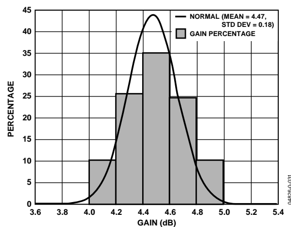
Figure 7. Conversion Gain Distribution, F_{RF} = 890 MHz, F_{IF} = 200 MHz
