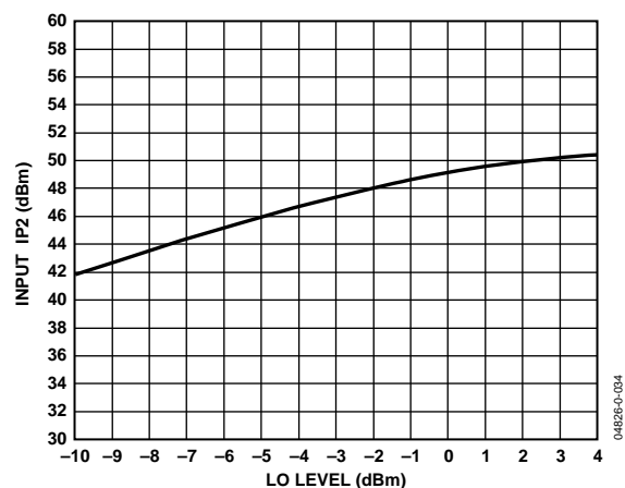
Figure 14. Input IP2 vs. LO Power, F_{RF} = 890 \text{ MHz} , F_{LO} = 1090 \text{ MHz} (RF Tone Spacing = 50 MHz)
