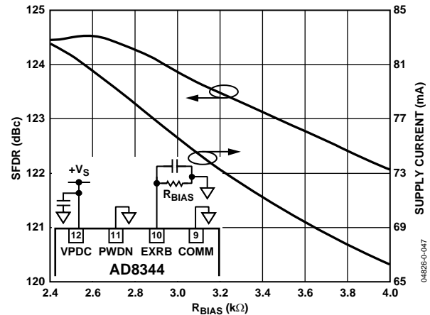
Figure 44. Impact of R_{BIAS} Resistor Selection vs. Spurious-Free Dynamic Range and Power Consumption, f_{RF} = 890\text{ MHz} and f_{LO} = 1090\text{ MHz}
