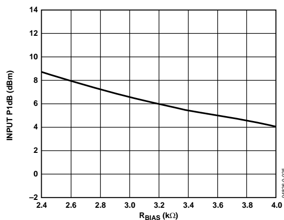
Figure 26. Input P1dB vs. R_{BIAS} , F_{RF} = 890 MHz, F_{LO} = 1090 MHz
