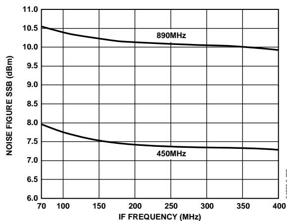
Figure 27. Noise Figure vs. IF Frequency
