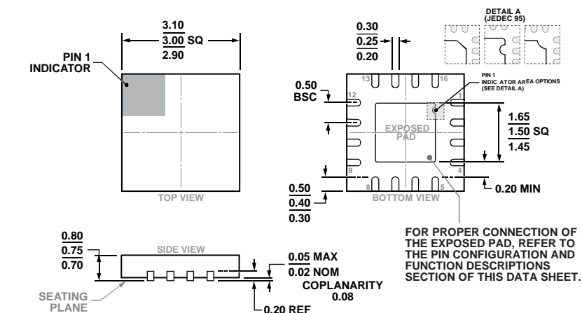
Figure 51. 16-Lead Lead Frame Chip Scale Package [LFCSP] 3 mm × 3 mm Body and 0.75 mm Package Height (CP-16-27)
