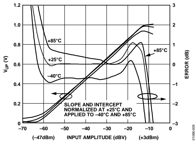
Figure 9. V_{UP} and Log Conformance vs. Input Amplitude at 2.5 GHz; -40°C, +25°C, and +85°C
