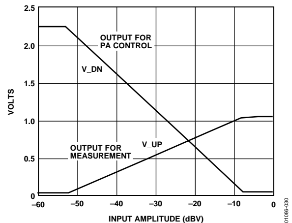
Figure 30. Showing V_{UP} and V_{DN} Relationship
