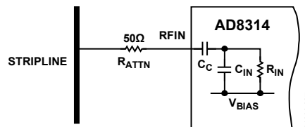
Figure 37. Series Attenuation
