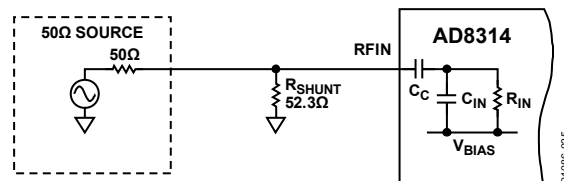
Figure 35. Broadband Resistive
