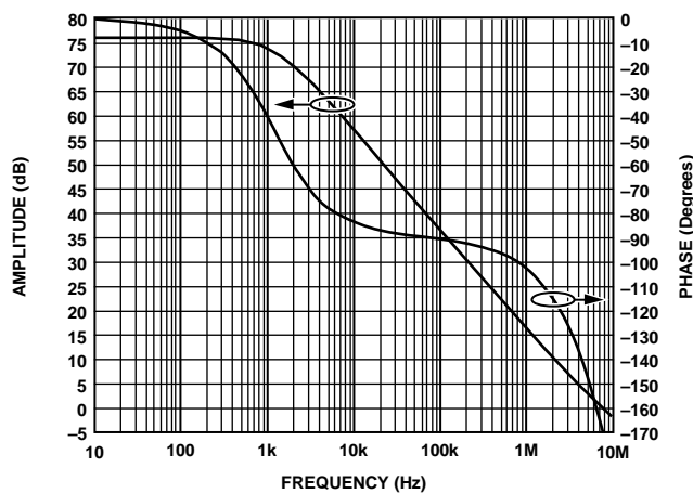
Figure 18. AC Response from VSET to V_{DN}
