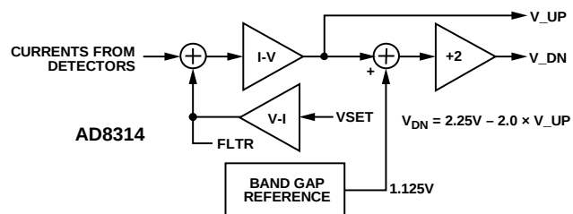
Figure 29. Output Interfaces
