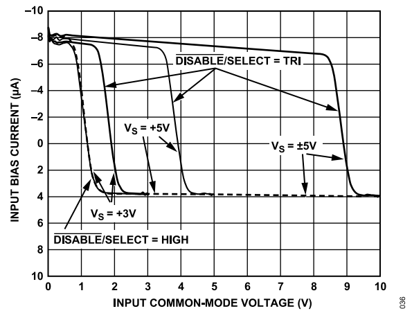
Figure 41. Input Bias Current vs. Input Common-Mode Voltage
