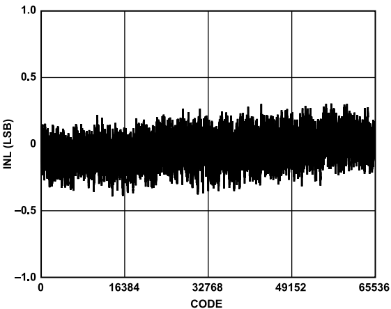
Figure 66. Integral Nonlinearity
