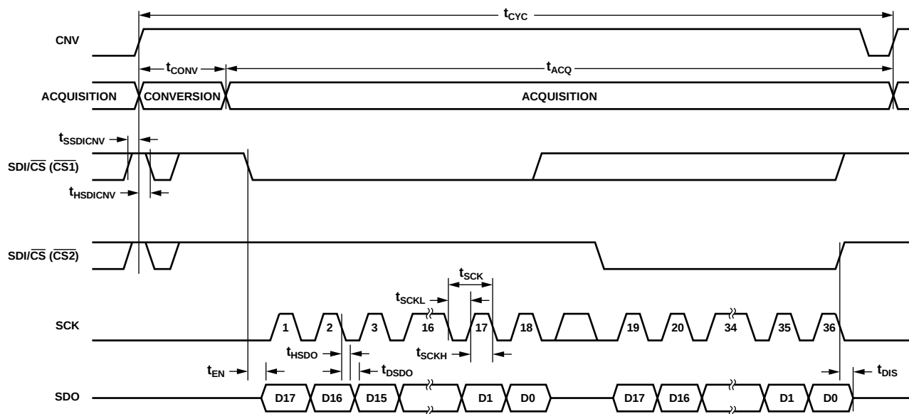
Figure 33. \overline{\text{CS}} Mode, 4-Wire Serial Interface Timing
