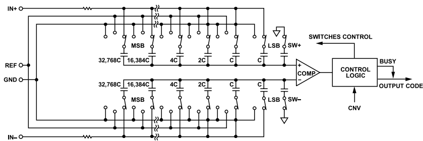
Figure 27. ADC Simplified Schematic
