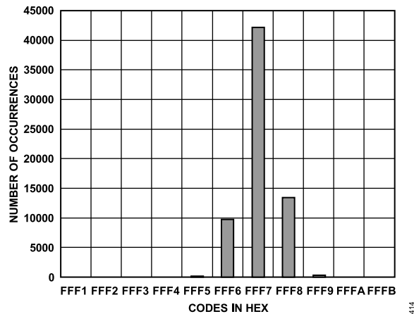
Figure 12. Histogram of a DC Input at the Code Center, REF = 2.5 V
