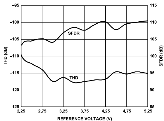
Figure 19. THD and SFDR vs. Reference Voltage
