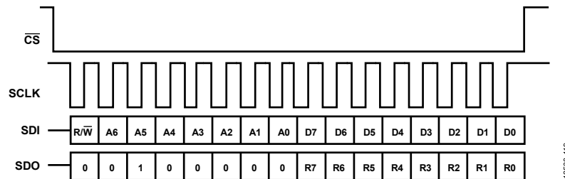
Figure 102. 16-Bit SPI Transfer—CRC Disabled
