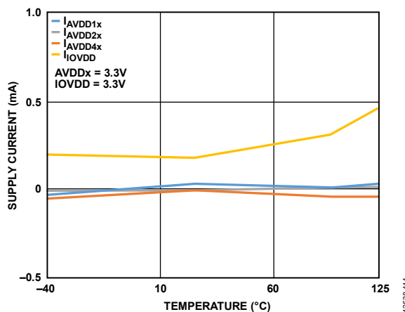
Figure 97. Shutdown Current
