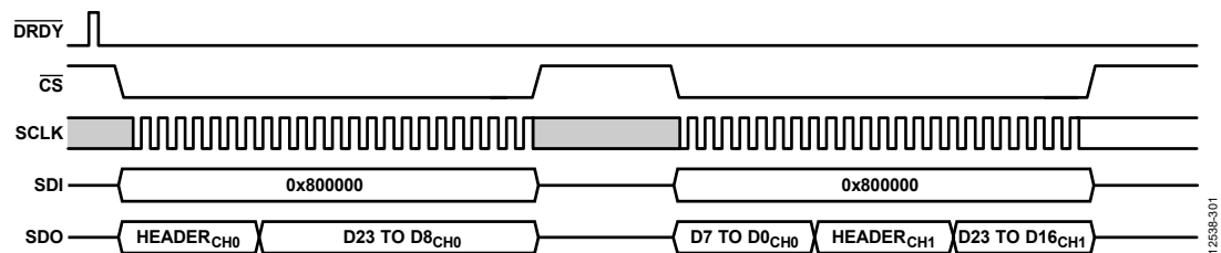
Figure 105. SPI Used to Read Back the \Sigma - \Delta ADC Data, in 24-Bit Frames
