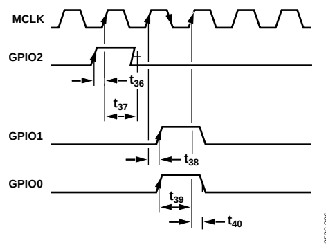
Figure 6. GPIOs for SRC Update Timing Diagram
