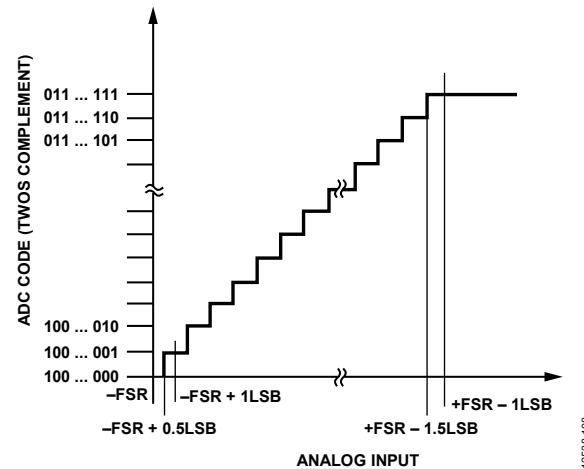
Figure 91. Transfer Function
