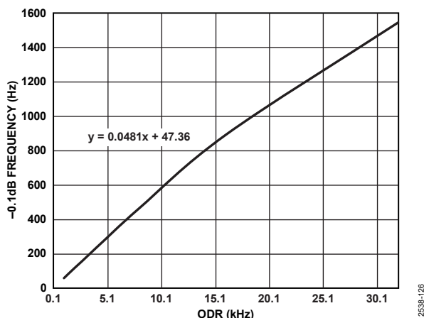
Figure 111. -0.1 dB Correction Factor
