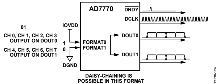
Figure 114. FORMATx Pin Configuration—FORMAT0 = 1, FORMAT1 = 0
