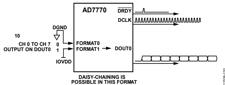
Figure 115. FORMATx Pin Configuration—FORMAT0 = 0, FORMAT1 = 1
