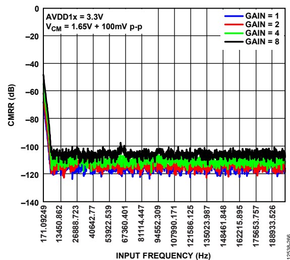
Figure 66. CMRR vs. Input Frequency at 4 kSPS, Low Power Mode
