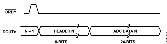
Figure 108. ADC Output—8-Bit Header Plus 24-Bit Conversion Data
