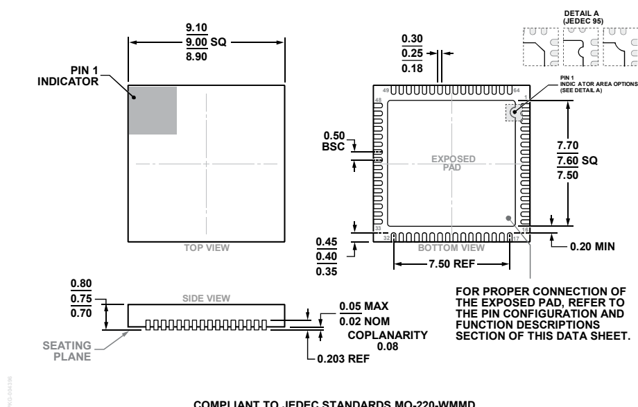
Figure 122. 64-Lead Lead Frame Chip Scale Package [LFCSP] 9 mm × 9 mm Body and 0.75 mm Package Height (CP-64-15) Dimensions shown in millimeters
