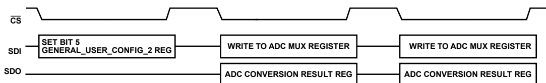
Figure 106. Configuring the AD7770 to Operate the SPI to Read from the SAR ADC
