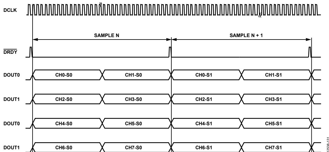
Figure 116. FORMAT0 = 0, FORMAT1 = 0—Each DOUTx Outputs Two ADC Conversions (S0 Means Sample 0 and S1 Means Sample 1)
