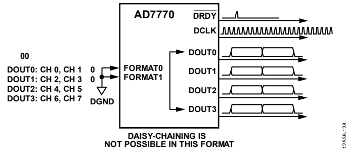
Figure 113. FORMATx Pin Configuration—FORMAT0 = 0, FORMAT1 = 0
