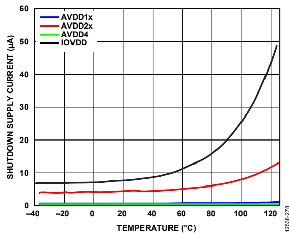
Figure 78. Shutdown Supply Current vs. Temperature
