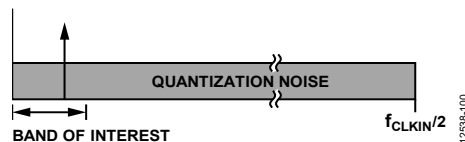
Figure 83. \Sigma - \Delta ADC Operation, Reduction of Noise Energy Contained in the Band of Interest (Linear Scale X-Axis)
