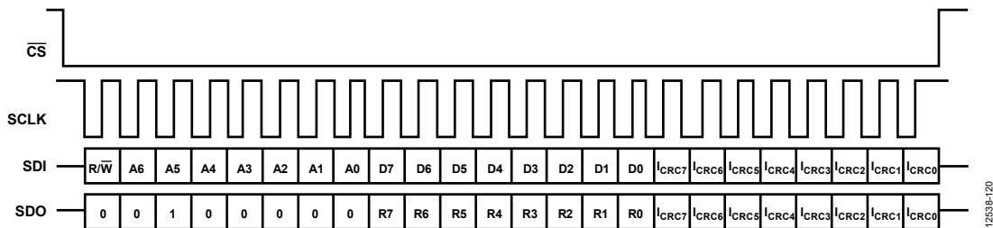
Figure 103. 24-Bit SPI Transfer—CRC Enabled
