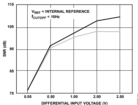
Figure 93. SNR Adding External LPF with V_{\text{REF}} = Internal Reference and f_{\text{CUTOFF}} < 10 Hz
