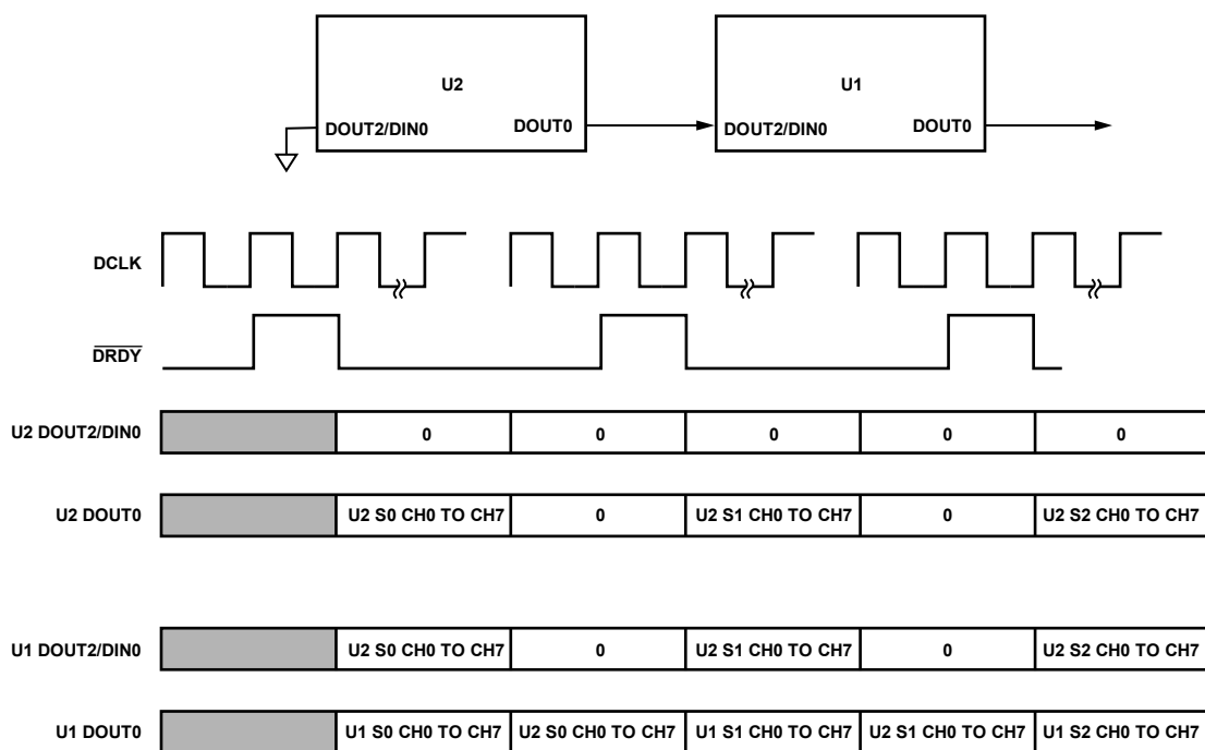
Figure 119. Daisy-Chain Connection Mode, FORMAT0 = 1, FORMAT1 = 0 (S0 Means Sample 0 and S1 Means Sample 1); When Connected in Daisy-Chain Mode, DOUT2 Acts as an Input Pin, Represented by DIN0
