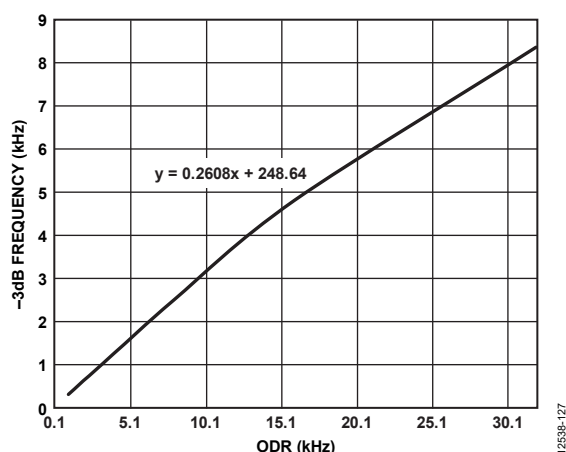
Figure 112. -3 dB Correction Factor
