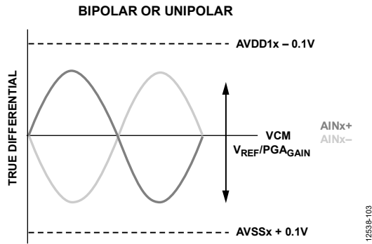
Figure 86. \Sigma - \Delta ADC Input Signal Configuration, True Differential
