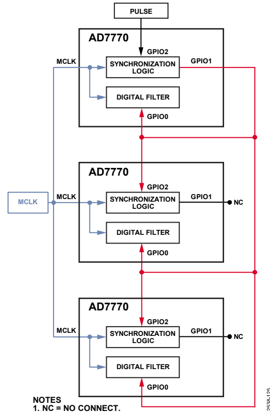
Figure 110. Hardware ODR Update
