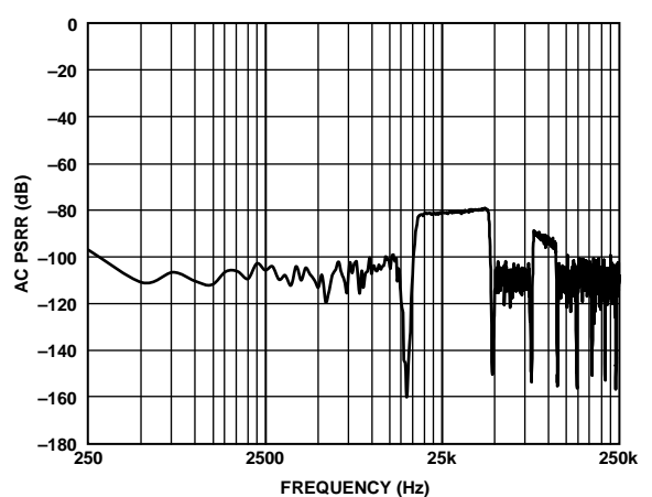
Figure 56. AVDD1 AC PSRR vs. Frequency, Low Power Mode, \text{AVDD1} = 5\text{ V} + 0.1\text{ V p-p}
