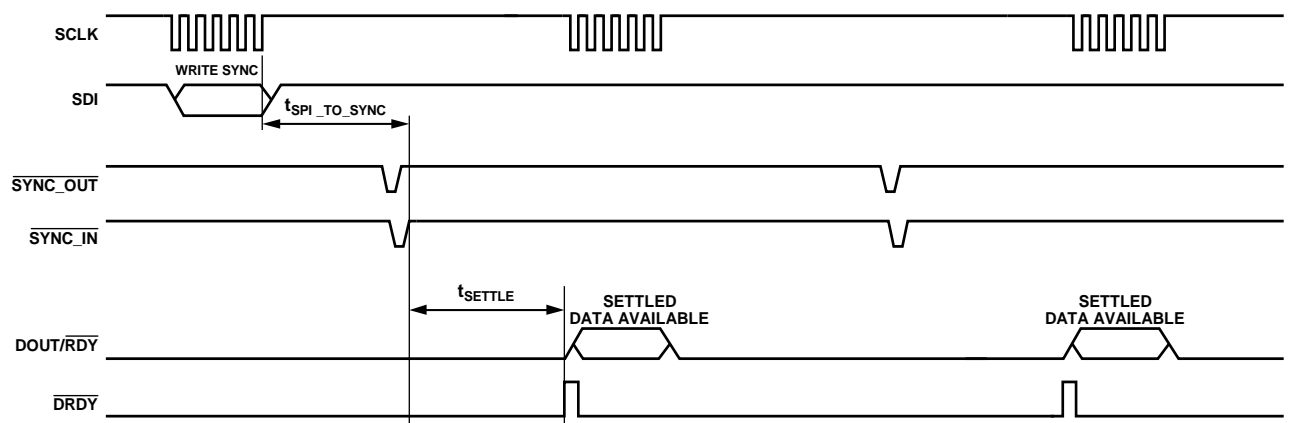
Figure 94. One Shot Conversion Mode, SYNC_IN Pulse Initiated by a Register Write
