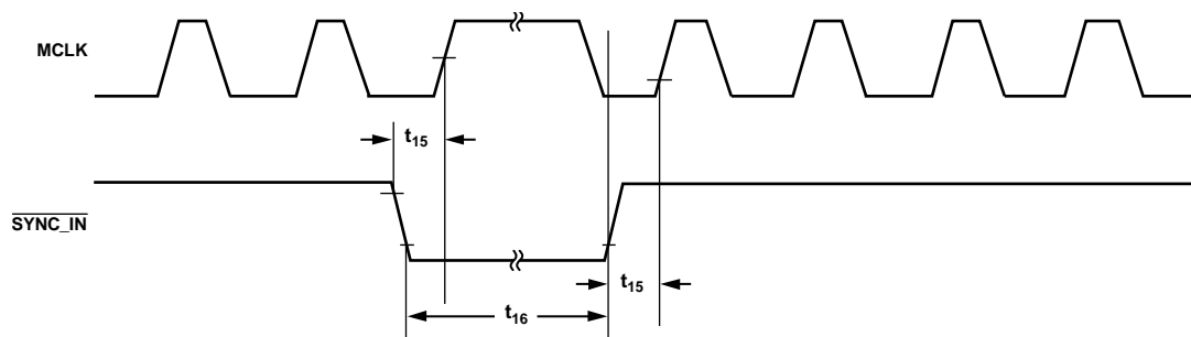
Figure 7. Synchronous SYNC_IN Pulse
