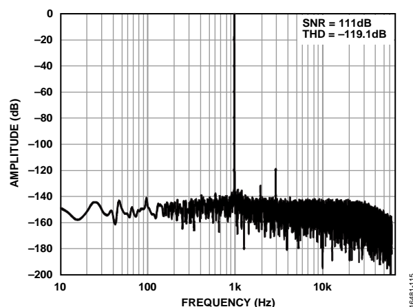
Figure 14. FFT, Median Mode, Sinc5 Filter, -0.25 dBFS
