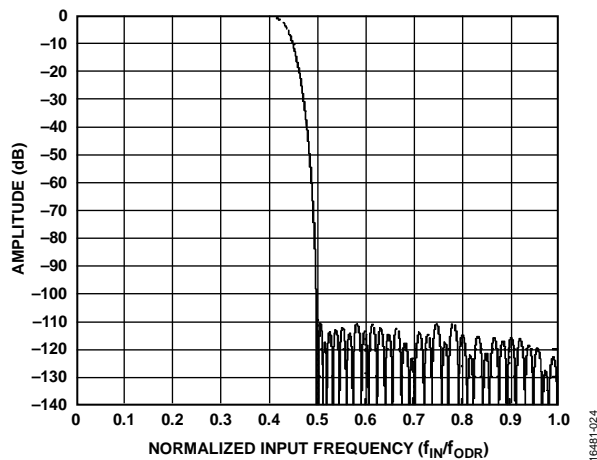
Figure 73. Low Ripple FIR Filter Frequency Response
