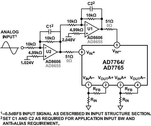
Figure 35. Driving the AD7765 Modulator Inputs Directly from a Single-Ended Source (On-Board Differential Amplifier Powered Down)
