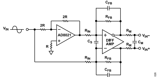
Figure 32. Single-Ended-to-Differential Conversion
