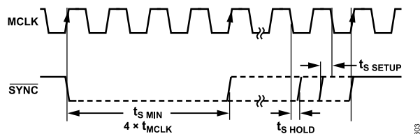
Figure 36. \overline{\text{SYNC}} Timing Relative to MCLK
