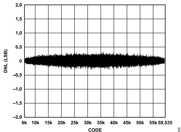
Figure 20. DNL Plot
