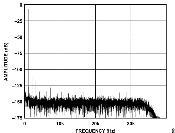
Figure 12. Normal Power Mode; FFT, 1 kHz, -6 dB Input Tone, 256× Decimation Rate
