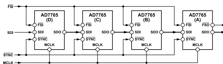
Figure 42. Writing to an AD7765 Daisy-Chain Configuration
