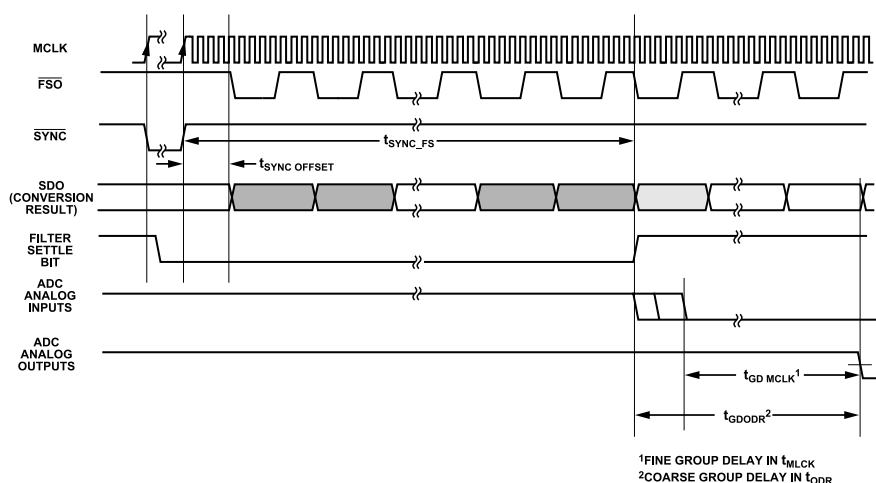
Figure 27. AD7765 Digital Filtering; Response to \overline{\text{SYNC}} , Settling Time, and Group Delay
