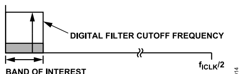
Figure 32. \Sigma - \Delta ADC, Digital Filter Cutoff Frequency
