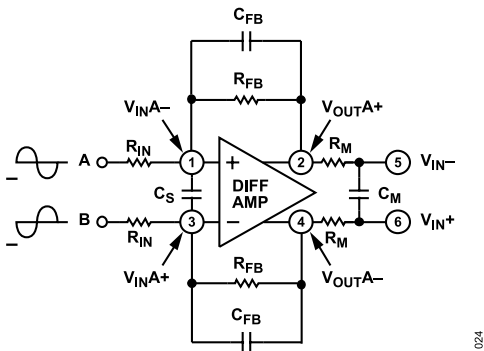
Figure 37. Differential Amplifier Configuration
