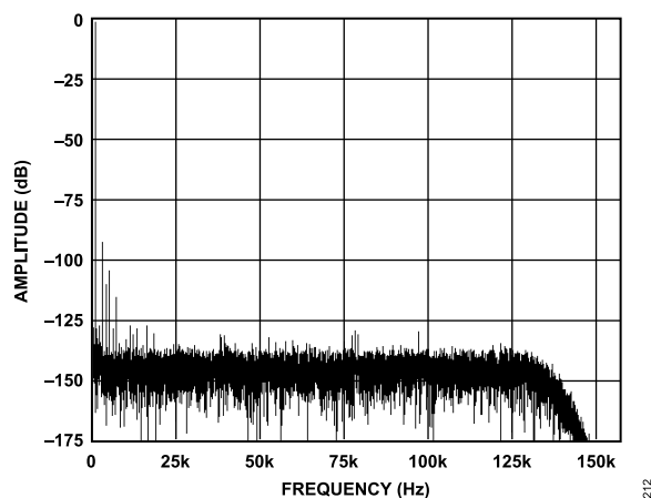
Figure 9. Low Power Mode, FFT, 1 kHz, -0.5\text{ dB} Input Tone, 64 \times Decimation Rate
