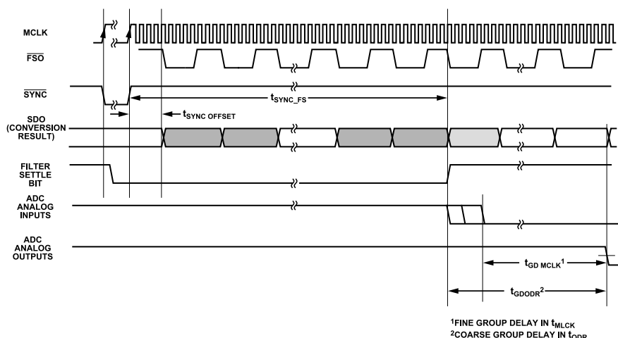
Figure 34. AD7764 Digital Filtering; Response to \overline{SYNC} , Settling Time, and Group Delay
