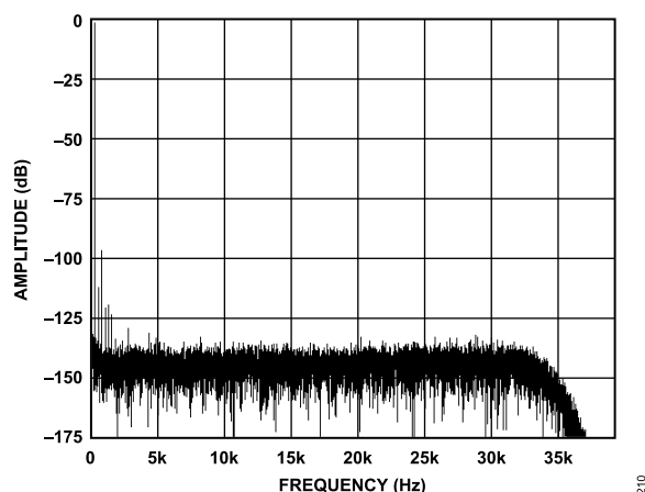
Figure 11. Low Power Mode, FFT, 1 kHz, -0.5\text{ dB} Input Tone, 256 \times Decimation Rate
