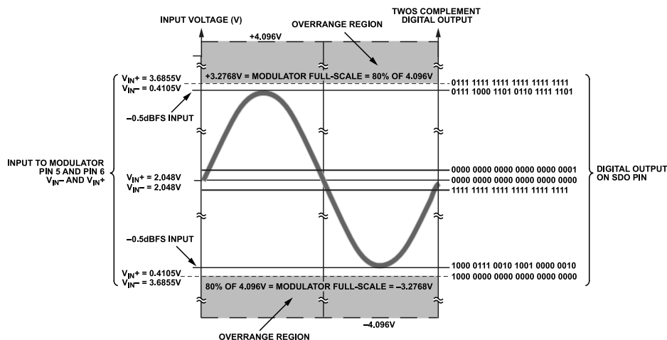
Figure 36. AD7764 Scaling: Modulator Input Voltage vs. Digital Output Code
