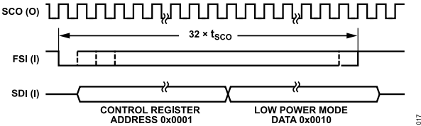
Figure 45. Write Scheme for Low Power Mode
