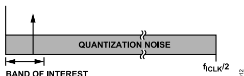
Figure 30. \Sigma - \Delta ADC, Quantization Noise
