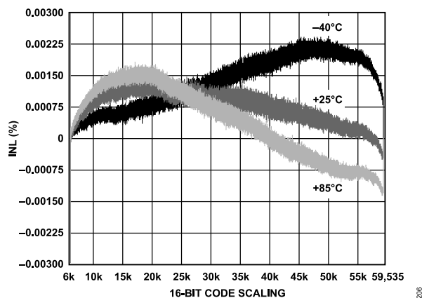
Figure 25. Normal Power Mode INL
