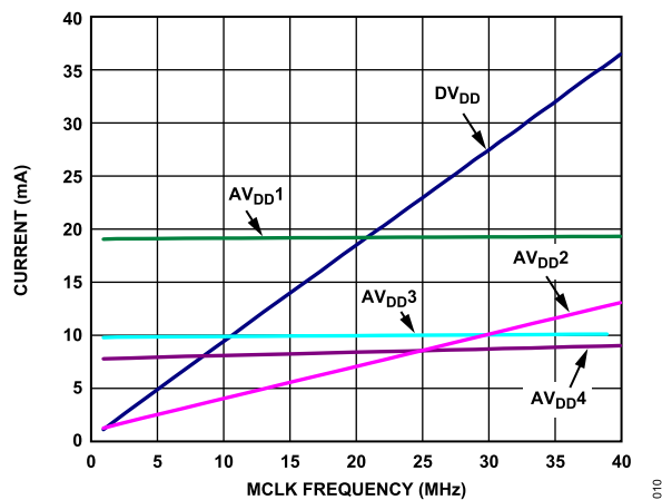
Figure 18. Normal Power Mode, Current Consumption vs. MCLK Frequency, 64x Decimation Rate
