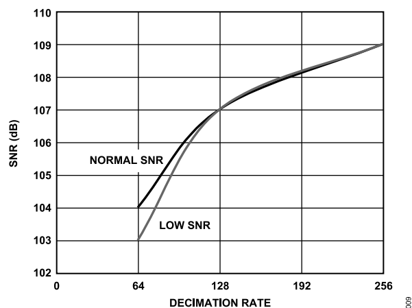
Figure 26. Normal and Low Power Mode, SNR vs. Decimation Rate, 1 kHz, -0.5 dB Input Tone
