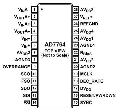
Figure 5. Pin Configuration
