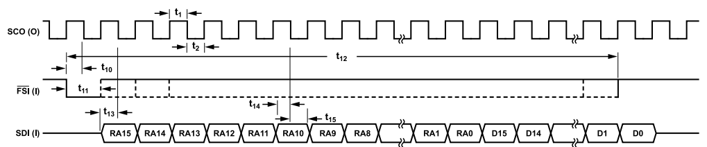
Figure 3. Register Write Timing Diagram
