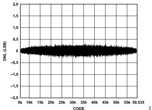
Figure 24. DNL Plot
