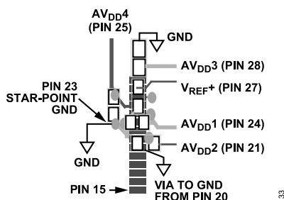
Figure 53. Supply Decoupling
