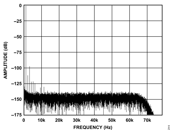
Figure 10. Low Power Mode, FFT, 1 kHz, -0.5\text{ dB} Input Tone, 128 \times Decimation Rate
