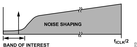
Figure 31. \Sigma - \Delta ADC, Noise Shaping
