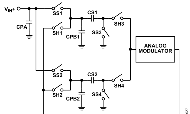
Figure 40. Equivalent Input Circuit
