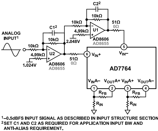
Figure 42. Driving the AD7764 Modulator Inputs Directly from a Single-Ended Source (On-Board Differential Amplifier Powered Down)
