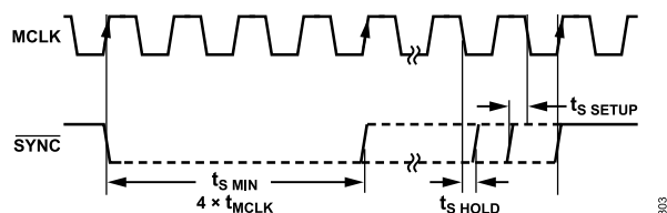
Figure 43. \overline{\text{SYNC}} Timing Relative to MCLK
