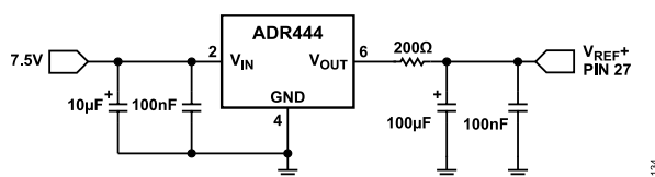
Figure 54. Reference Connection
