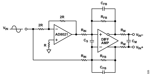
Figure 39. Single-Ended to Differential Conversion
