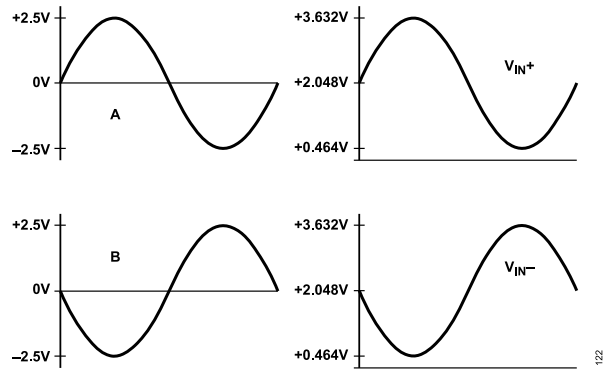
Figure 38. Differential Amplifier Signal Conditioning
