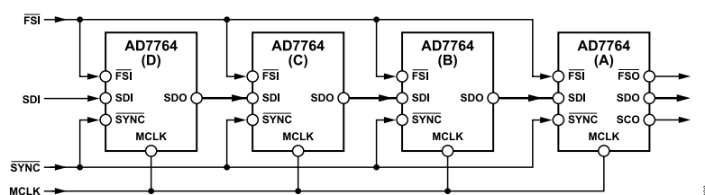
Figure 49. Writing to an AD7764 Daisy-Chain Configuration
