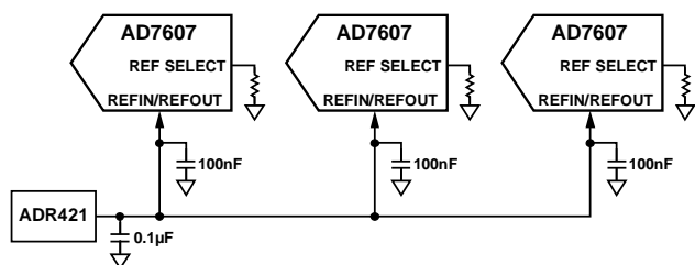
Figure 37. Single External Reference Driving Multiple AD7607 REFIN Pins
