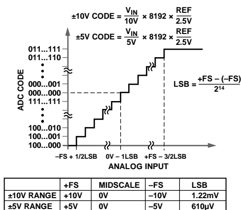
Figure 35. Transfer Characteristics
