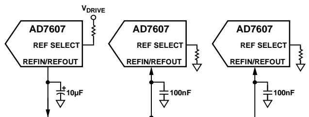
Figure 38. Internal Reference Driving Multiple AD7607 REFIN Pins.
