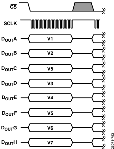
Figure 106. Serial Interface ADC Reading, Eight DOUTX Lines
