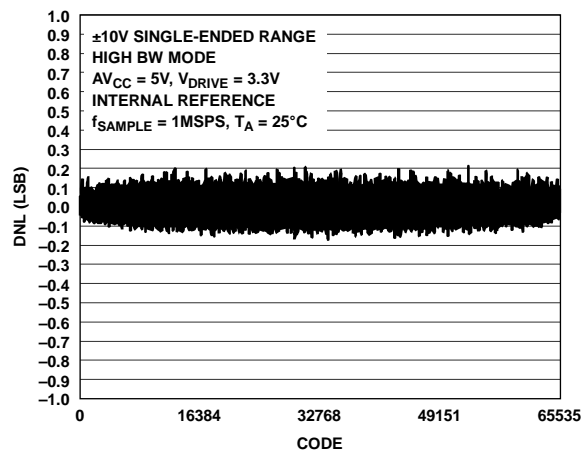
Figure 42. Typical DNL, High Bandwidth Mode
