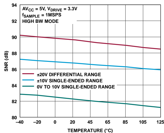
Figure 44. SNR vs. Temperature, High Bandwidth Mode
