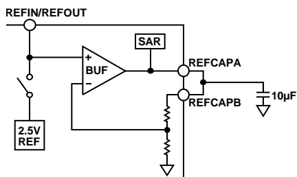
Figure 83. Reference Circuitry
