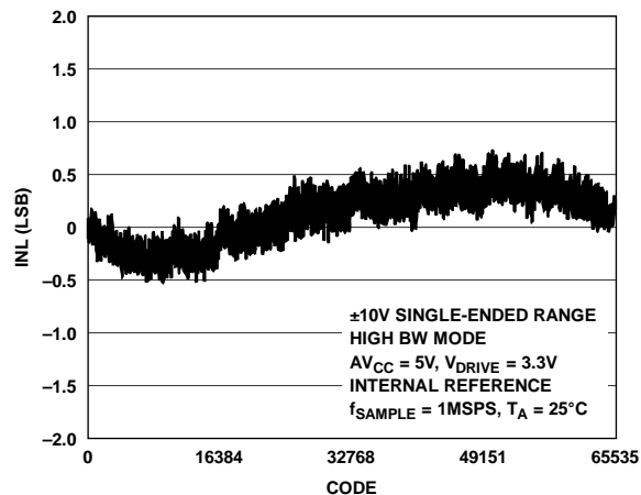
Figure 43. Typical INL, High Bandwidth Mode
