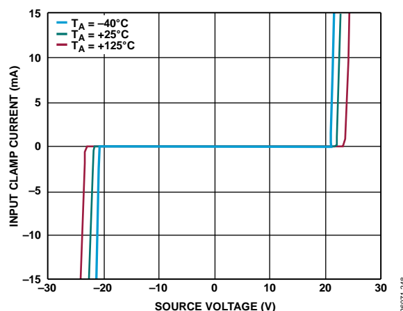
Figure 75. Input Protection Clamp Profile
