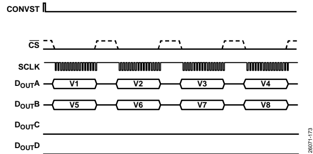
Figure 104. Serial Interface ADC Reading, Two DOUTX Lines
