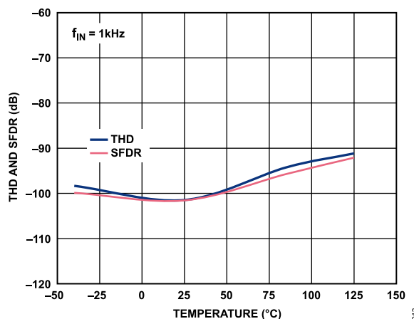
Figure 17. AD7403 THD and SFDR vs. Temperature
