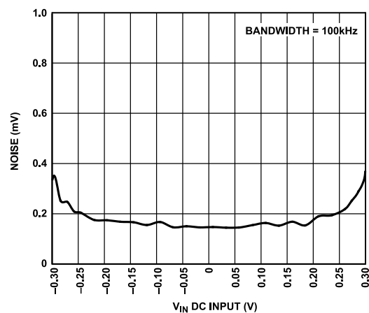
Figure 17. RMS Noise Voltage vs. V_{IN} DC Input
