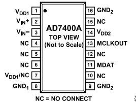
Figure 5. Pin Configuration
