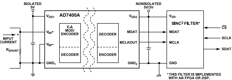
Figure 21. Typical Application Circuit
