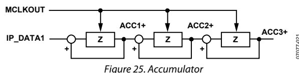
Figure 25. Accumulator
