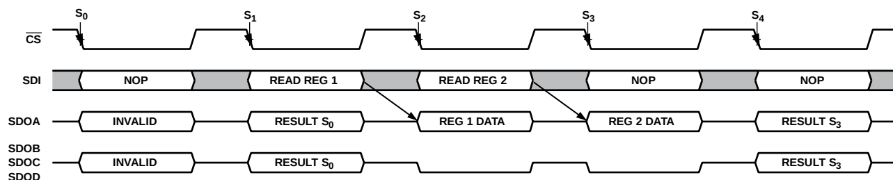
Figure 40. Register Read
