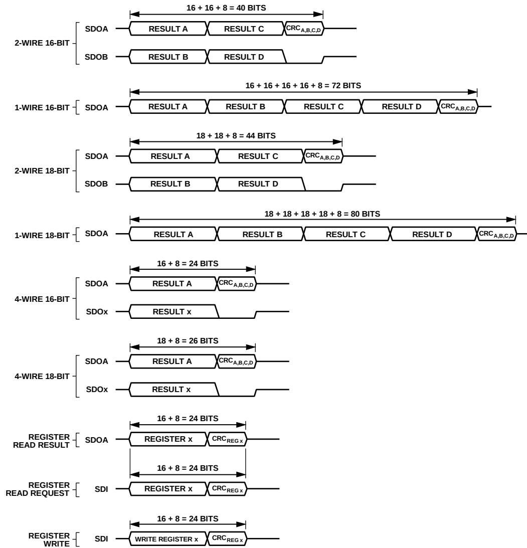
Figure 42. CRC Operation
