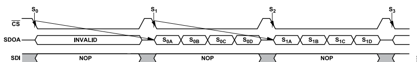
Figure 37. Reading Conversion Results, 1-Wire Mode
