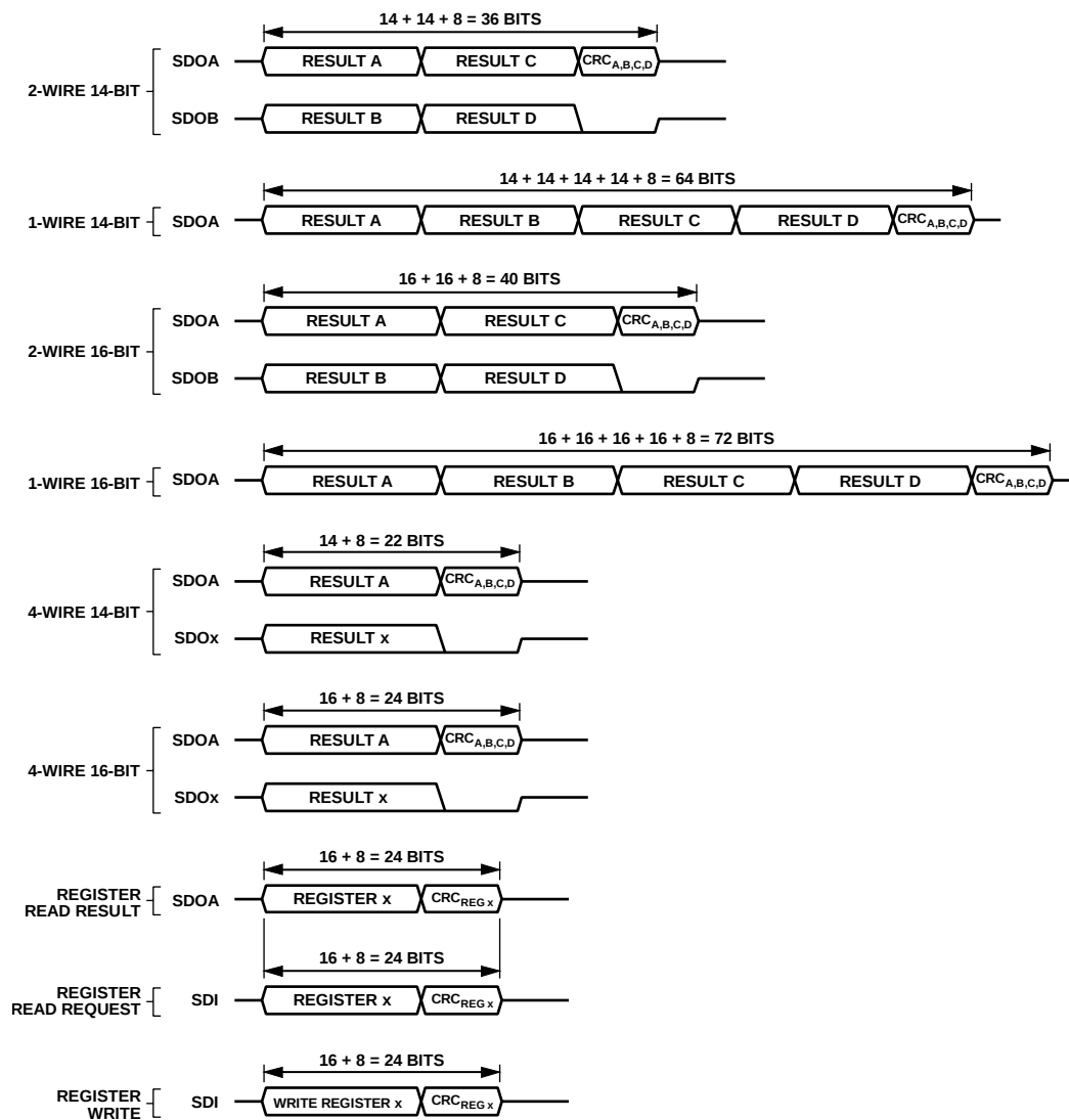
Figure 44. CRC Operation
