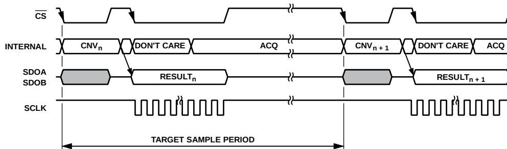
Figure 41. Low Throughput Low Latency
