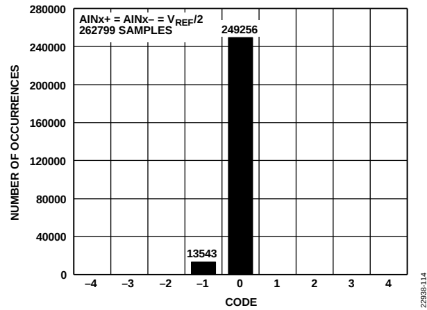
Figure 14. Code Histogram
