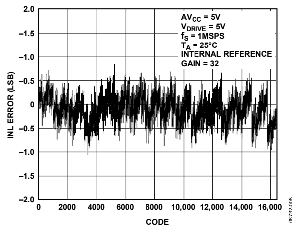
Figure 9. Typical INL at Gain of 32
