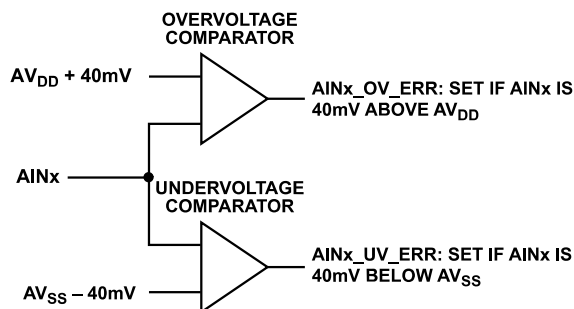
Figure 119. Analog Input Overvoltage/Undervoltage Monitors
