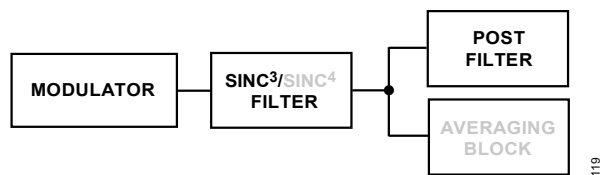
Figure 109. Post Filters
