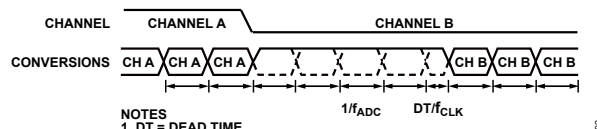
Figure 82. Sinc 4 Channel Change
