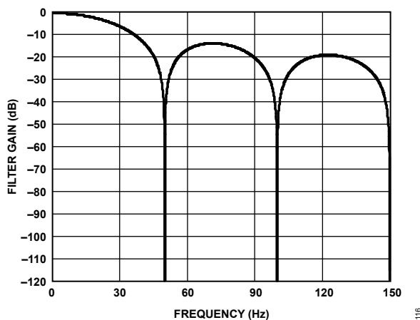
Figure 106. 50 Hz Rejection
