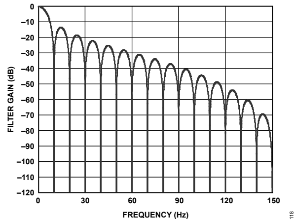
Figure 108. Simultaneous 50 Hz and 60 Hz Rejection
