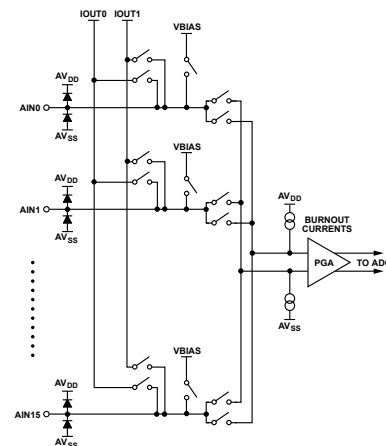
Figure 77. Excitation Current and Bias Voltage Connections
