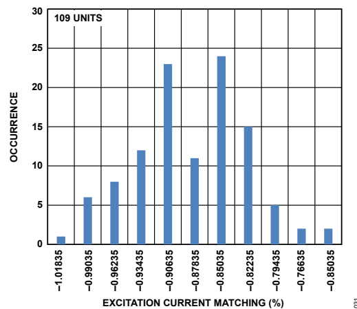
Figure 31. IOUTx Current Initial Matching Histogram (500 µA)
