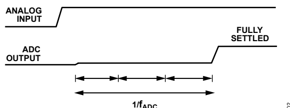
Figure 92. \text{Sinc}^3 Zero Latency Operation
