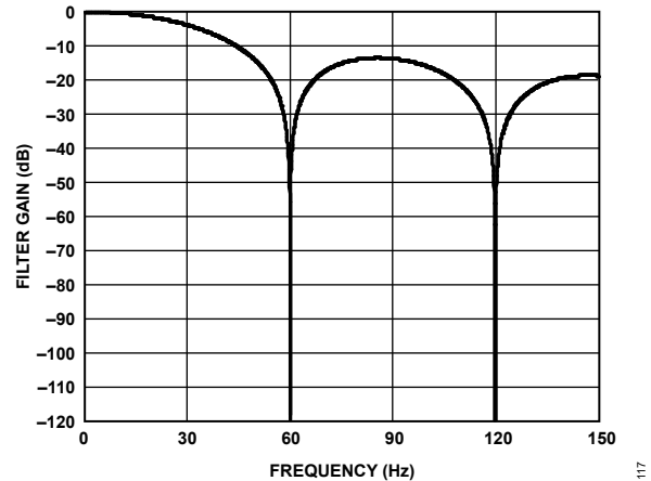
Figure 107. 60 Hz Rejection
