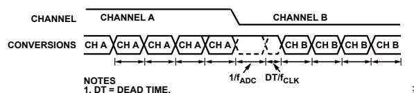
Figure 104. Fast Settling, \text{Sinc}^3 + \text{Sinc}^1 Filter
