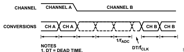
Figure 90. Sinc 3 Channel Change
