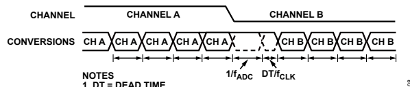
Figure 98. Fast Settling, Sinc 4 + Sinc 1 Filter
