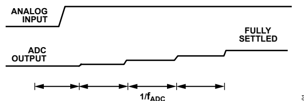
Figure 91. Asynchronous Step Change in the Analog Input
