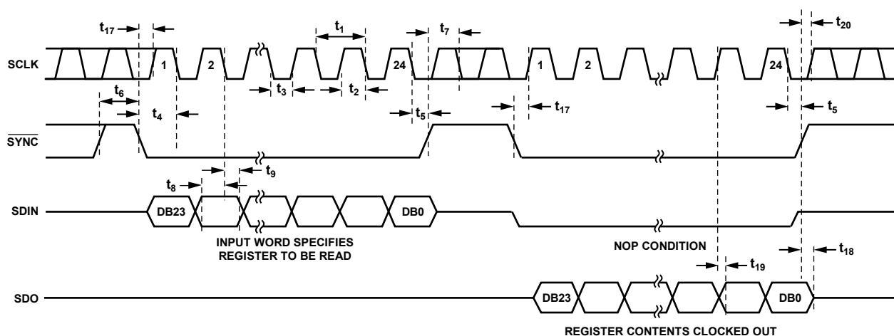
Figure 3. Readback Mode Timing Diagram
