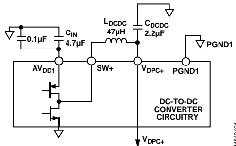
Figure 77. DC-to-DC Circuit
