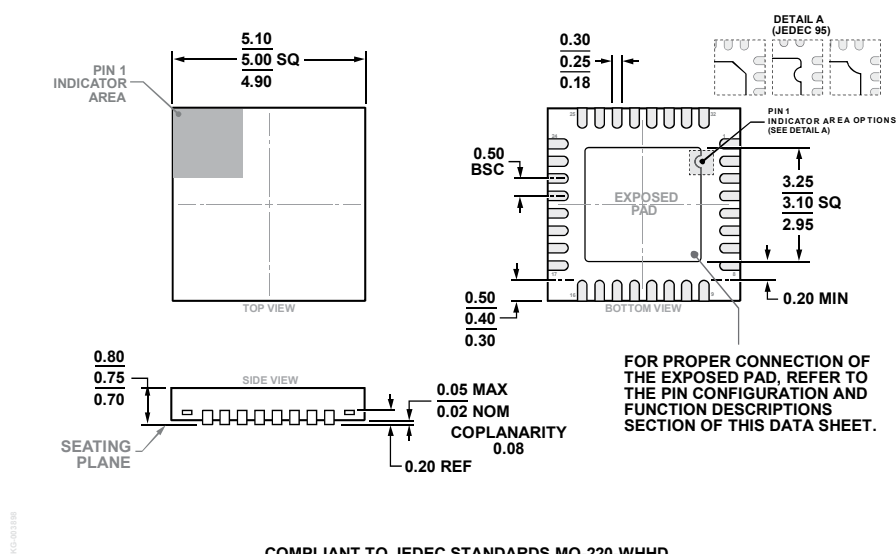
Figure 58. 32-Lead Lead Frame Chip Scale Package [LFCSP] 5 mm × 5 mm Body and 0.75 mm Package Height (CP-32-7)
