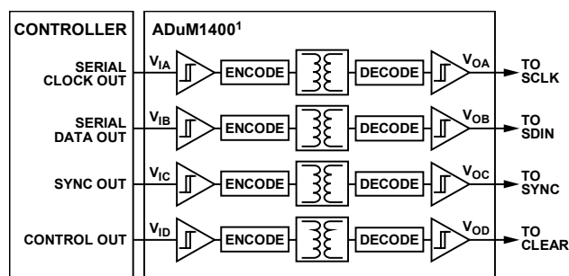
Figure 57. Isolated Interface
