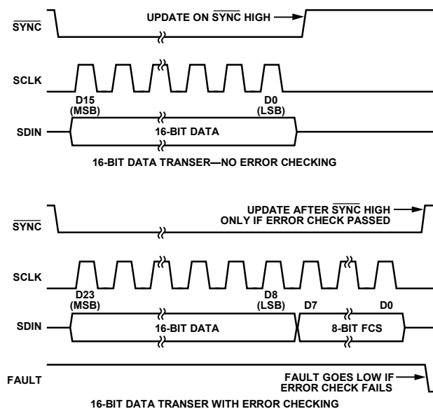
Figure 54. PEC Error Checking Timing
