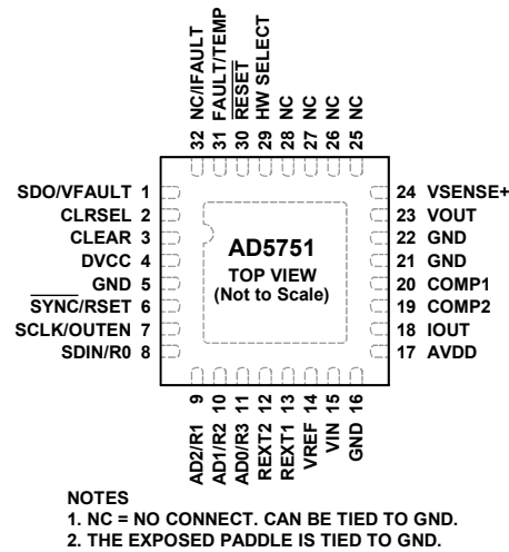
Figure 4. Pin Configuration
