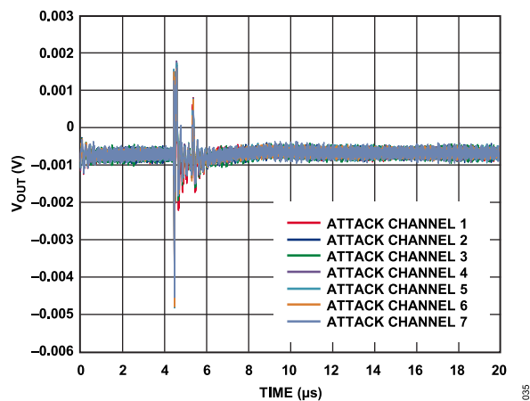
Figure 33. Analog Crosstalk
