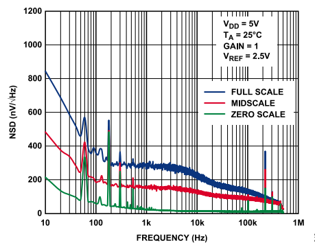
Figure 36. Noise Spectral Density (NSD)
