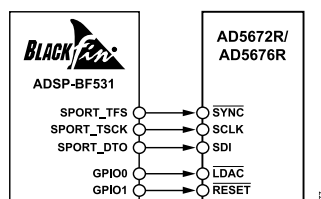
Figure 70. SPORT Interface
