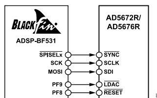
Figure 69. ADSP-BF531 Interface
