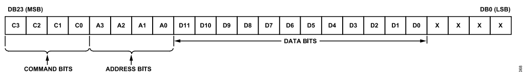
Figure 60. AD5672R Input Shift Register Content
