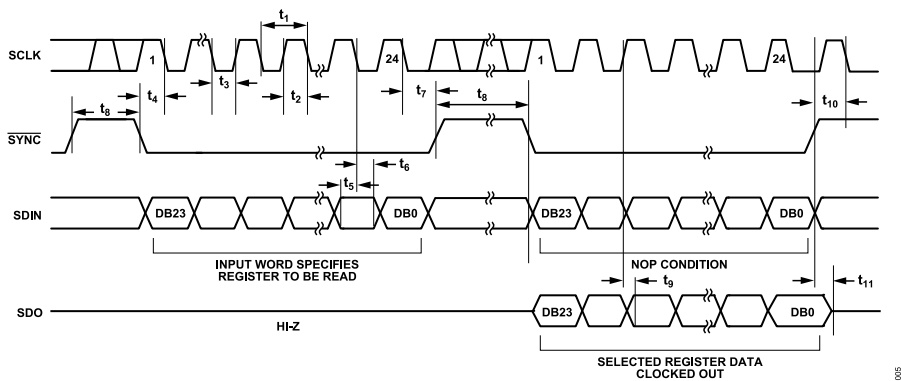
Figure 5. Readback Timing Diagram
