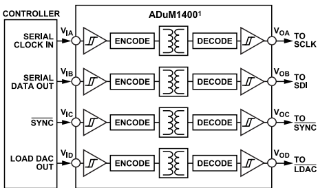
Figure 72. Isolated Interface
