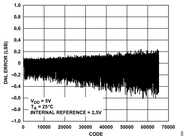
Figure 11. AD5676R DNL Error vs. Code
