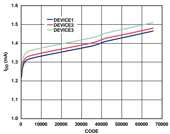
Figure 35. I_{DD} vs. Code
