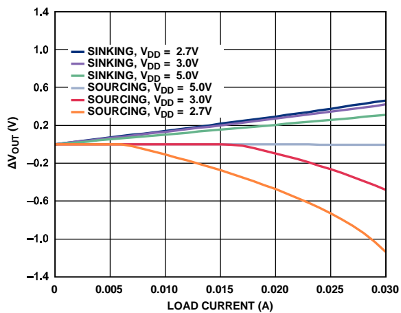
Figure 32. Output Voltage Change ( \Delta V_{out} ) vs. Load Current
