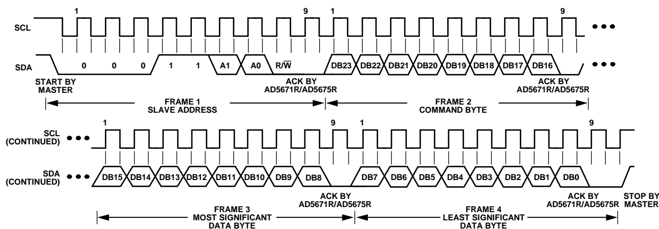
Figure 59. I 2 C Write Operation
