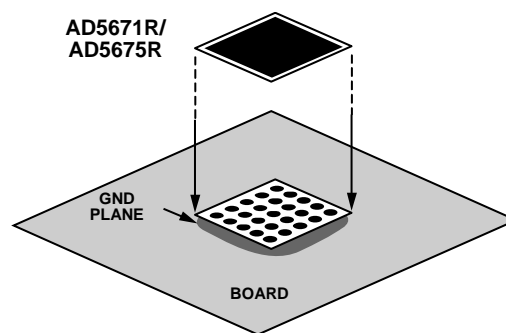
Figure 68. Pad Connection to Board
