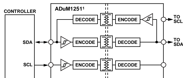
Figure 69. Isolated Interface
