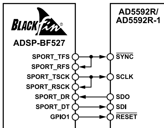
Figure 52. ADSP-BF527 SPORT Interface
