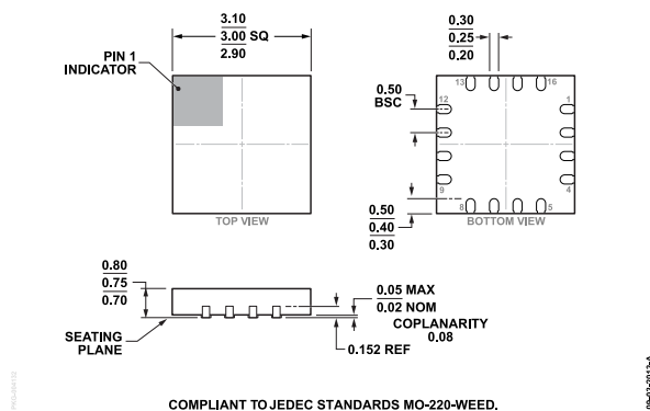
Figure 54. 16-Lead Lead Frame Chip Scale Package [LFCSOP] 3 mm × 3 mm Body, Very Very Thin Quad (CP-16-32) Dimensions shown in millimeters
