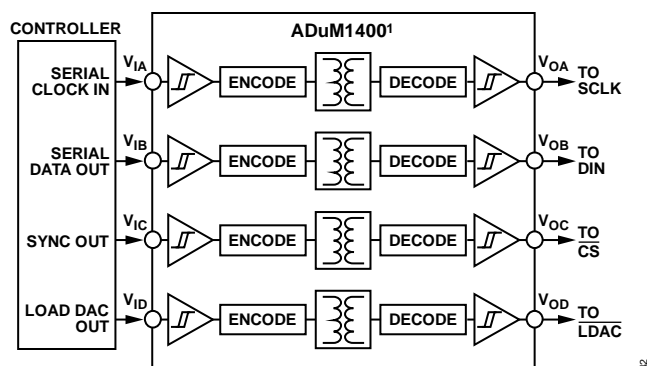
Figure 34. Isolated Interface
