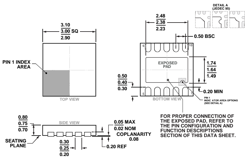
Figure 37. 10-Lead Lead Frame Chip Scale Package [LF CSP] 3 mm x 3 mm Body and 0.75 mm Package Height (CP-10-9)
