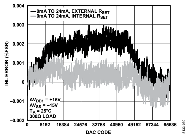
Figure 25. INL Error vs. DAC Code
