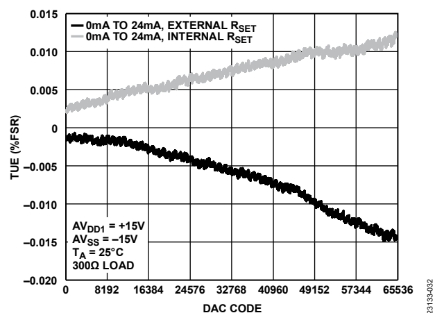
Figure 27. TUE vs. DAC Code
