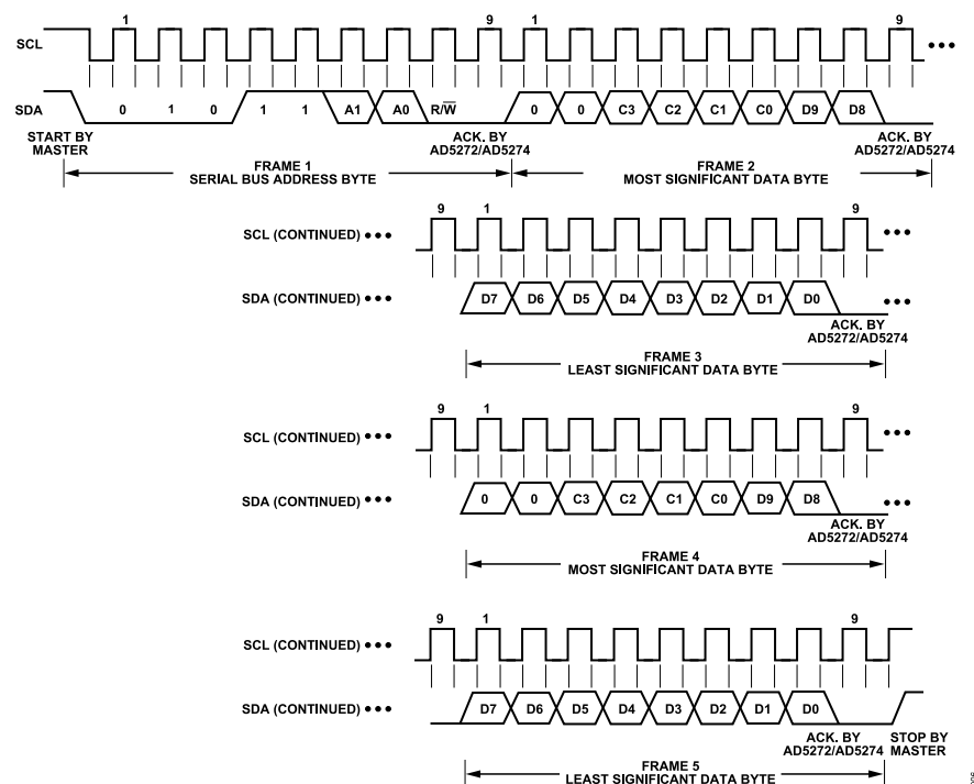
Figure 44. Multiple Write
