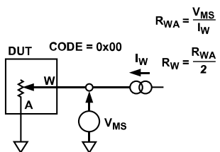
Figure 39. Wiper Resistance
