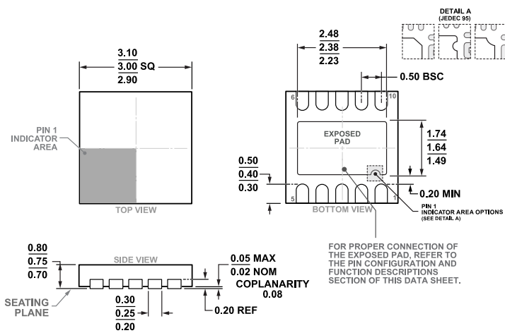
Figure 50. 10-Lead Frame Chip Scale Package [LFCSP] 3 mm × 3 mm Body and 0.75 mm Package Height (CP-10-9) Dimensions shown in millimeters
