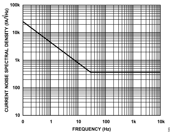
Figure 20. Input Current Noise vs. Frequency
