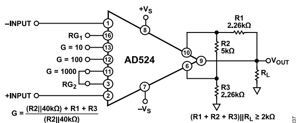
Figure 37. Gain of 2000
