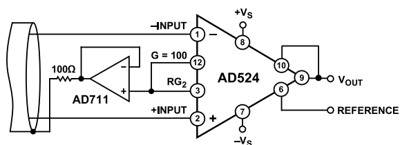
Figure 41. Shield Driver, G \geq 100
