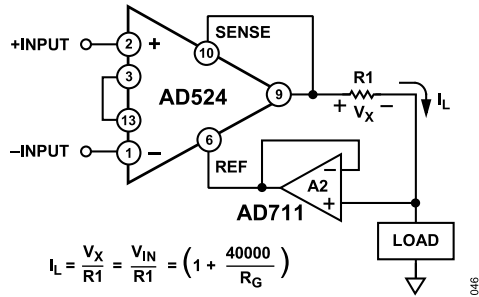
Figure 46. Voltage-to-Current Converter
