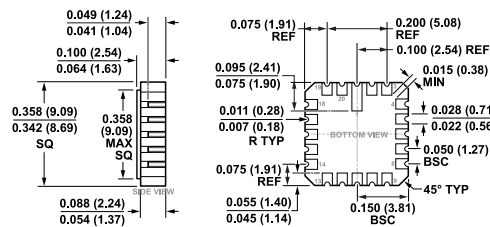
Figure 56. 20-Terminal Ceramic Leadless Chip Carrier [LCC] (E-20-1)
