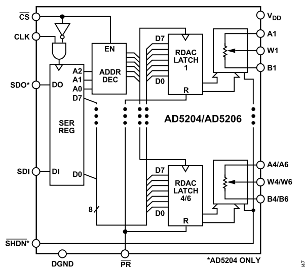
Figure 32. Block Diagram
