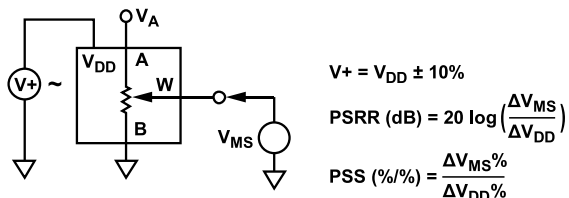
Figure 26. Power Supply Sensitivity Test Circuit (PSS, PSRR)
